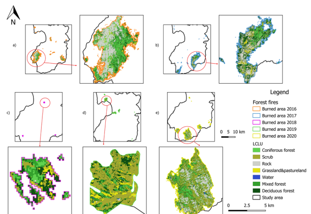
Figure 6. LCLU classes located in the burned areas (a) 2016-year (b) 2017 year; (c) 2018 year; (d) 2019 year; (e) 2020 year.
