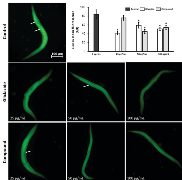
Fig. 3 Effect of glz or [Pd(glz) 2 ] compound treatment on A \beta accumulation. A \beta accumulation was identified in transgenic C. elegans (CL4176) stained with thioflavin T. Arrows indicate the representative A \beta aggregation deposits in untreated worms. The bar chart represents the fluorescence intensity of the representative worms from each group ( n = 15 ). * means statistical differences ( P < 0.059 ) with respect to 0 \mu\text{g mL}^{-1} in the control group.
