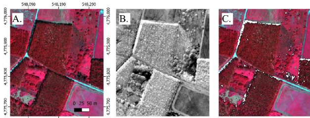
Figure 2. Example of shadow removal. A. Original WorldView image in false color infrared (B8, B5, B3). B. Shadow Detection Index (SDI) (Shahi et al., 2014). C. New raster with shadow data defined as NULL, represented as white pixels.
