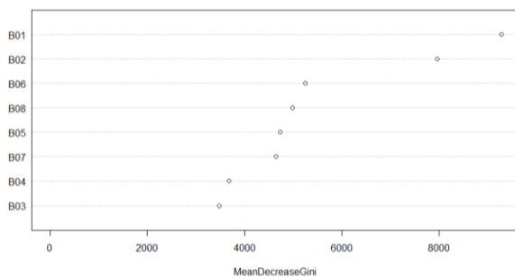
Figure 5. Plot of the Mean Decrease in Gini for each of the WorldView bands used in the prediction. B01: Coastal Blue; B02: Blue; B03: Green; B04: Yellow; B05: Red; B06: Red Edge; B07: NIR1; B08: NIR2.
