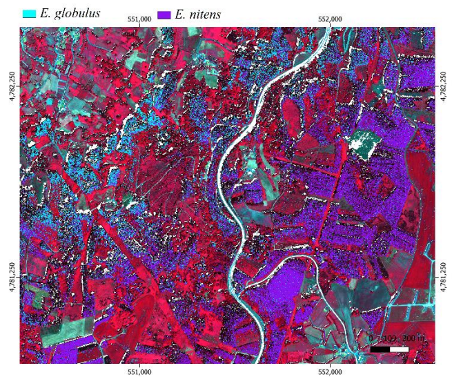
Figure 4. Example of result of the Eucalyptus species classification. Reference image WorldView image in false color infrared (B8, B5, B3). White correspond to shadowed areas.
