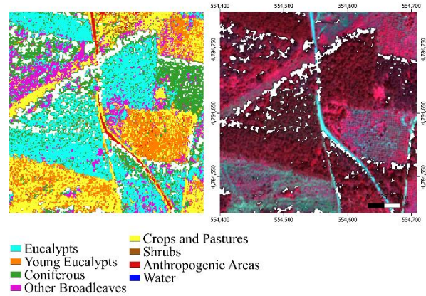
Figure 3. On the left: results of the general classification. On the right: reference WorldView image in false color infrared (B8, B5, B3). White areas in both images correspond to shadowed areas.
