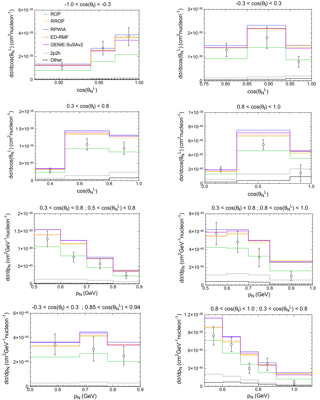
FIG. 4. T2K CC0 \pi semi-inclusive \nu_\mu - {}^{12}\text{C} cross section with protons in the final state with momenta above 0.5 GeV as a function of the final proton and muon kinematics. All curves include the 2p2h and pion absorption contributions (also shown separately), evaluated using GENIE. Cross section measurements taken from [1].
