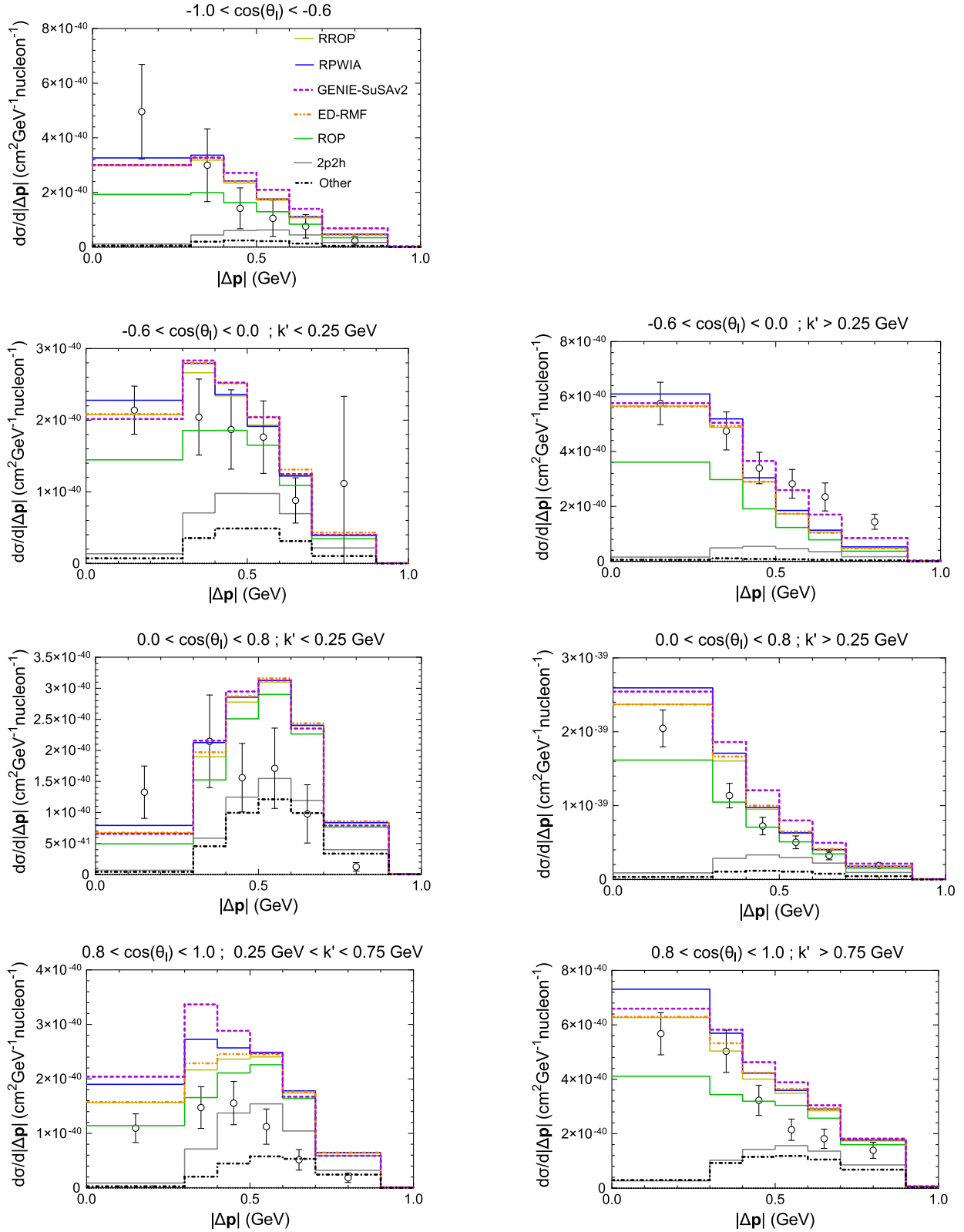
FIG. 8. T2K CC0 \pi semi-inclusive \nu_\mu - {}^{12}\text{C} cross section as function of the variable |\Delta p| defined in Eq. (11) in different muon kinematic bins with constrains of the proton kinematics given in Table II. All curves include the 2p2h and pion absorption contributions (also shown separately), evaluated using GENIE. Cross section measurements taken from [1].
