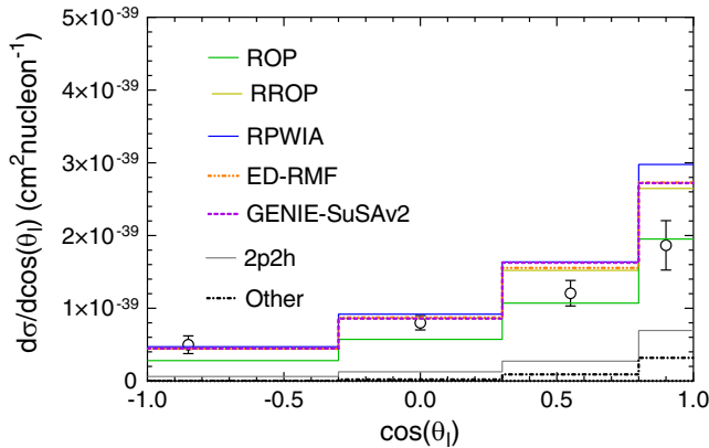
FIG. 5. T2K CC0\pi semi-inclusive \nu_\mu - {}^{12}\text{C} cross section with protons in the final state with momenta above 0.5 GeV as function of the muon scattering angle. All curves include the 2p2h and pion absorption contributions (also shown separately), evaluated using GENIE. Cross section measurements taken from [1].
