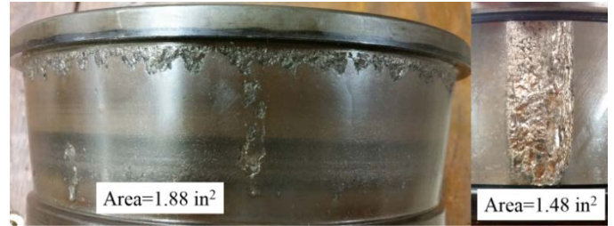
Figure 10. Photographs depicting large defects (spalls) present on bearing inner ring (cone) raceways.
