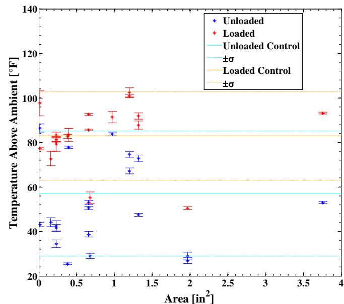
Figure 9. Temperature data of bearings with outer ring defects of various sizes (as measured by defect area) compared against the range of operating temperatures for healthy (control) bearings for unloaded (17% load) and loaded (100% load) conditions at a speed of 60 mph.
