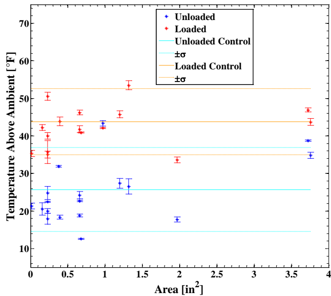
Figure 8. Temperature data of bearings with outer ring defects of various sizes (as measured by defect area) compared against the range of operating temperatures for healthy (control) bearings for unloaded (17% load) and loaded (100% load) conditions at a speed of 30 mph.
