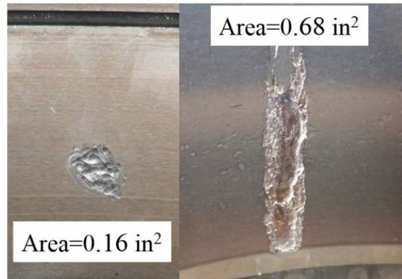
Figure 11. Photographs depicting small (left) and medium (right) size defects (spalls) present on bearing outer ring (cup) raceways.
