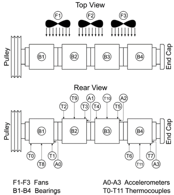
Figure 3. Schematic showing the top and rear view of the dynamic bearing tester, including sensor locations.
