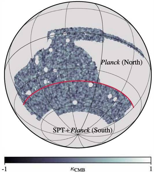
FIG. 1. Upper: Diagram illustrating the input temperature maps used to construct the two different lensing maps utilized in this analysis. The operation “QE” (quadratic estimator) is the lensing reconstruction step described in Section IID 2. Lower: Illustration of the sky coverage and lensing maps for the North ( Planck ) and South ( SPT+Planck ) patches. The red line indicates the cut in declination ( \text{dec} = -40^\circ ) that divides the two regions. The union of the DES mask used in the DES Y3 analysis and the Planck lensing map mask is applied.
