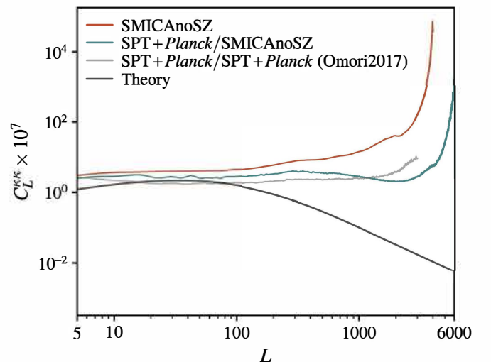
FIG. 3. Noise levels estimated from simulations for SPT+Planck/SMICAnoSZ (teal) and Planck (orange) over the patch of sky that will be used to measure the cross-correlations. Also shown are the noise levels from [20] (light gray) and an analytical prediction for the convergence signal (black). The procedures described in Section II D eliminate tSZ contamination from the lensing maps at the cost of a small increase in the map noise (teal vs. light gray).
