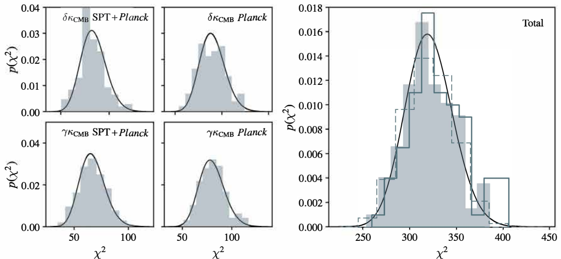
FIG. 10. Left : Distribution of \chi^2 derived from FLASK simulations and our covariance model for \langle \delta_g \kappa_{\text{CMB}} \rangle and \langle \gamma_t \kappa_{\text{CMB}} \rangle data vectors in the SPT+ Planck and Planck patches separately. The histograms are overlaid with a \chi^2_\nu distribution (smooth black curve), and we only include data points after the scale cuts (see Section V). Right : Same as the left panel but for the combined data vector of \langle \delta_g \kappa_{\text{CMB}} \rangle and \langle \gamma_t \kappa_{\text{CMB}} \rangle in both patches (filled histogram). The open gray histogram represents the \chi^2 distribution prior to applying the 4% correction and the dashed histogram corresponds to the \chi^2 distribution when combining different realizations for the SPT+ Planck and Planck patches, effectively nulling the off-diagonal block of the covariance in the FLASK realizations, as described in Section IV B 2
