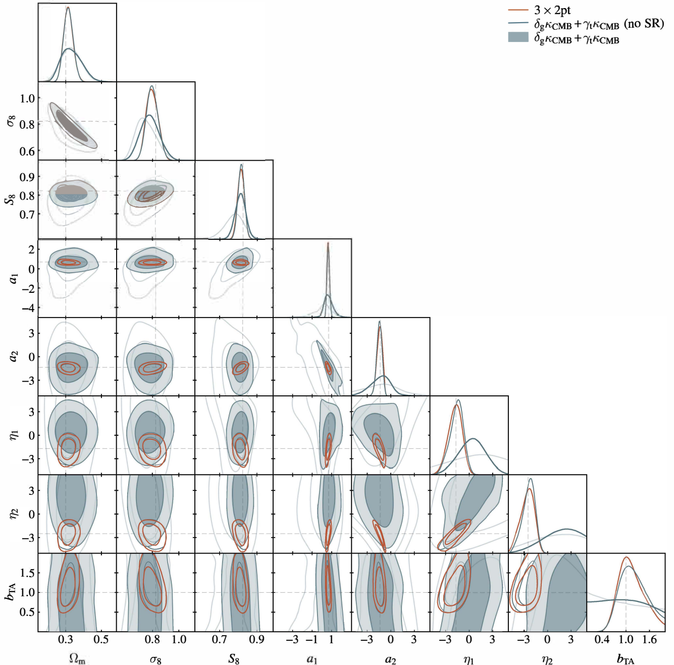
FIG. 13. Comparison of the forecasted constraints on cosmological parameters \Omega_m, \sigma_8, S_8 and intrinsic alignment parameters a_1, a_2, \eta_1, \eta_2 , and b_{\text{TA}} using the combination of galaxy clustering and galaxy-CMB lensing correlation, with and without the addition of shear-ratio information, compared with the constraints from 3 \times 2\text{pt} . The dashed lines represent the input values for the individual parameters.
