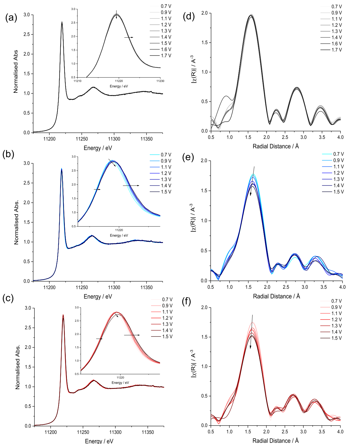
Figure 5. In situ normalized XANES spectra for (a) r-IrO 2 , (b) IrO x , and (c) Li-IrO x recorded at different electrode potentials in 0.1 M HClO 4 . Insets show an expansion of the absorption peak to highlight the change in position. Fourier-transformed Ir EXAFS spectra of (d) r-IrO 2 , (e) IrO x and (f) Li-IrO x at given electrode potentials.
