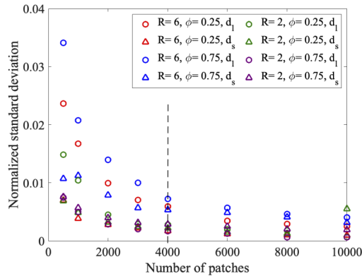
Fig. 4. Variation of normalised standard deviation as a function of the number of patches averaged from DEM simulation data.
