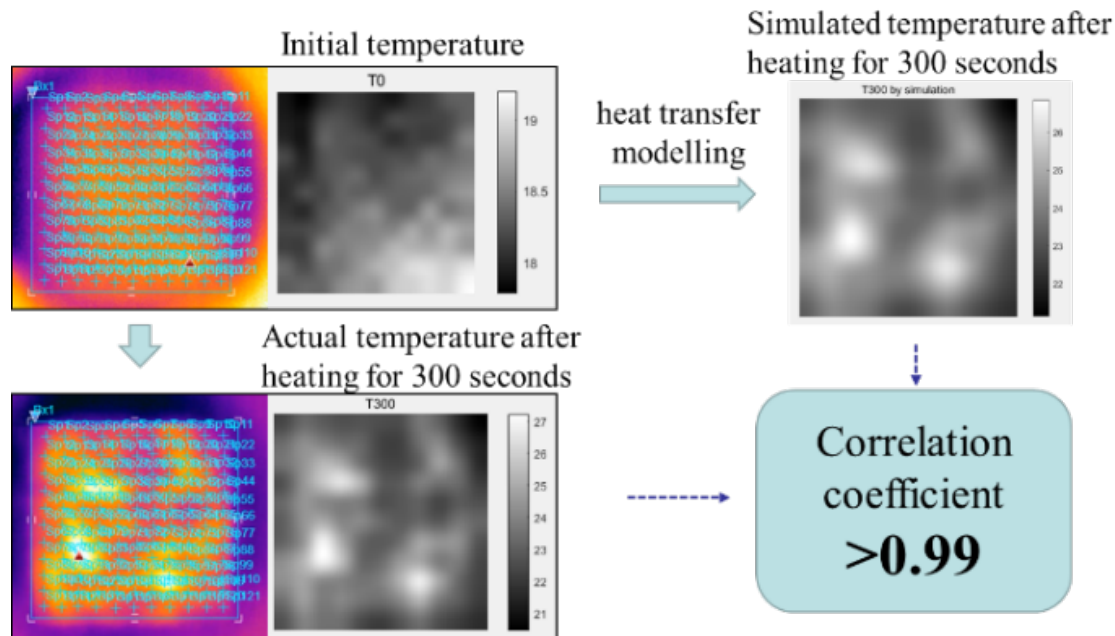
Figure 2. Accuracy evaluation for heat transfer model using image based programming.
