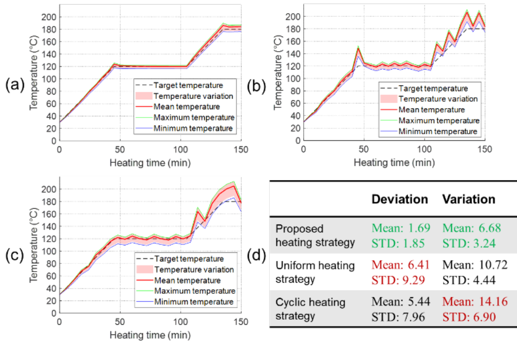
Figure 4. Results of simulation: (a) proposed heating strategy; (b) uniform heating strategy; (c) cyclic heating strategy; (d) deviation and variation of induced temperature w.r.t target profile.
