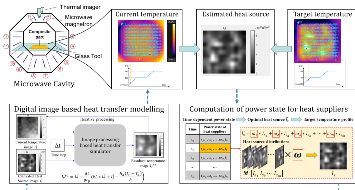
Figure 1. An overview of the numerical thermal control method for composite curing process using digital image based programming.
