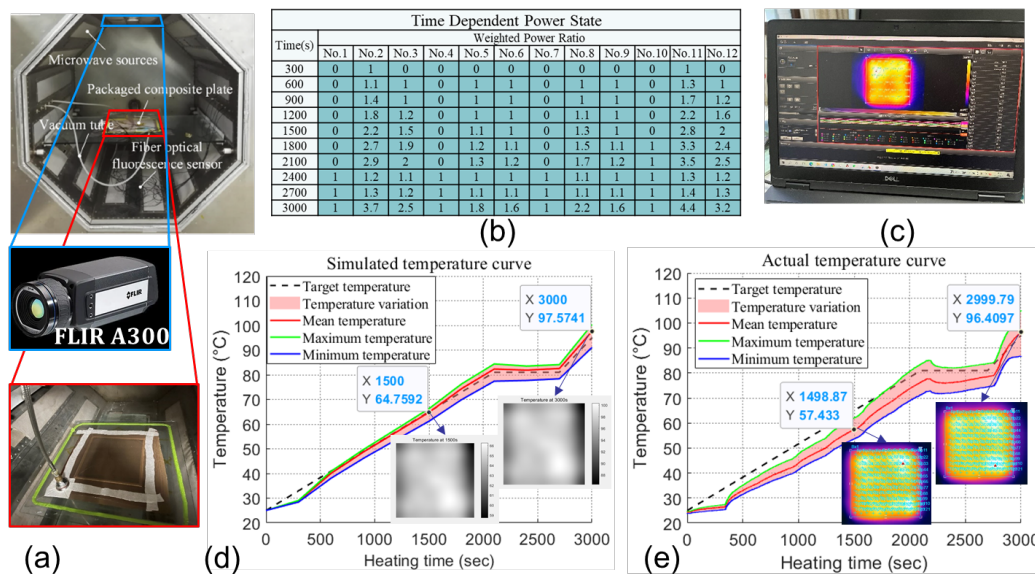
Figure 5. Results of actual heating: (a) experimental setup; (b) optimized power state; (c) heating process; (d) simulation result; (e) actual result.
