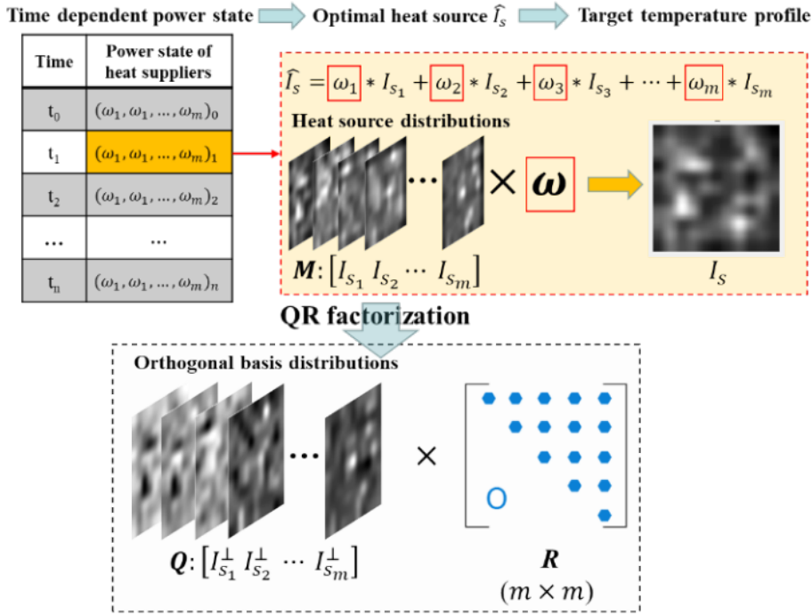
Figure 3. Computation of time dependent power state.
