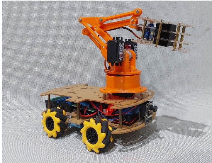
Figure 10. Testing a Robot Arm Holding an Object
