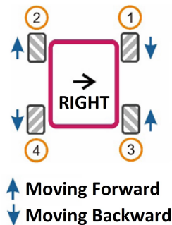
Figure 8. Mecanum wheel configuration
