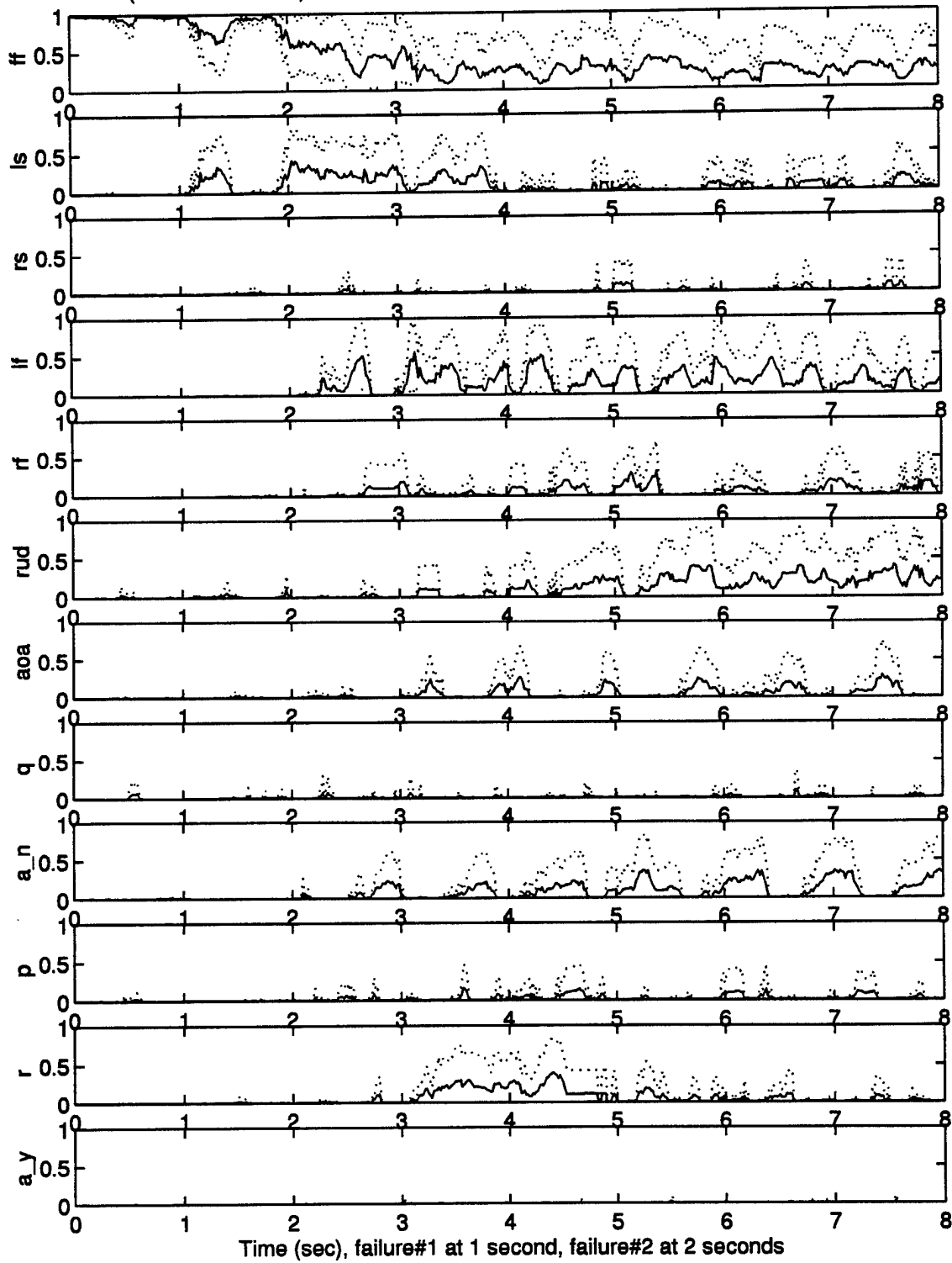
Mean (+/- One Std Dev) Dual-fail Probabilities of fail501.503 with reconfiguration: 10 runs
