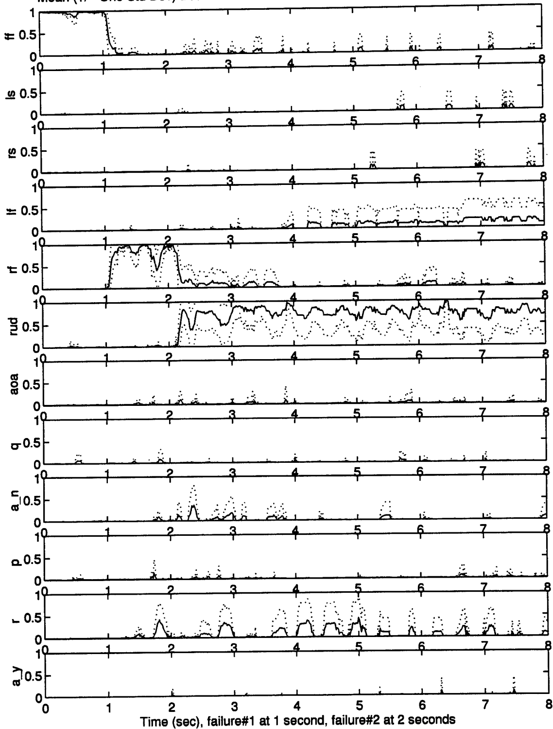
Mean (+/- One Std Dev) Dual-fail Probabilities of fail254.255 with reconfiguration: 10 runs
