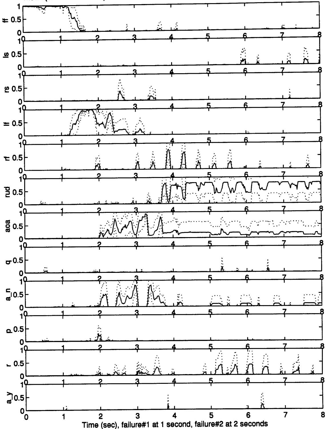
Mean (+/- One Std Dev) Dual-fail Probabilities of fail253.06 with reconfiguration: 10 runs
