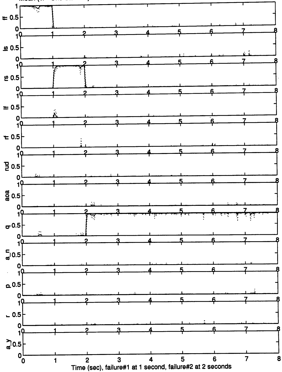
Mean (+/- One Std Dev) Dual-fail Probabilities of fail002.007 with reconfiguration: 10 runs
