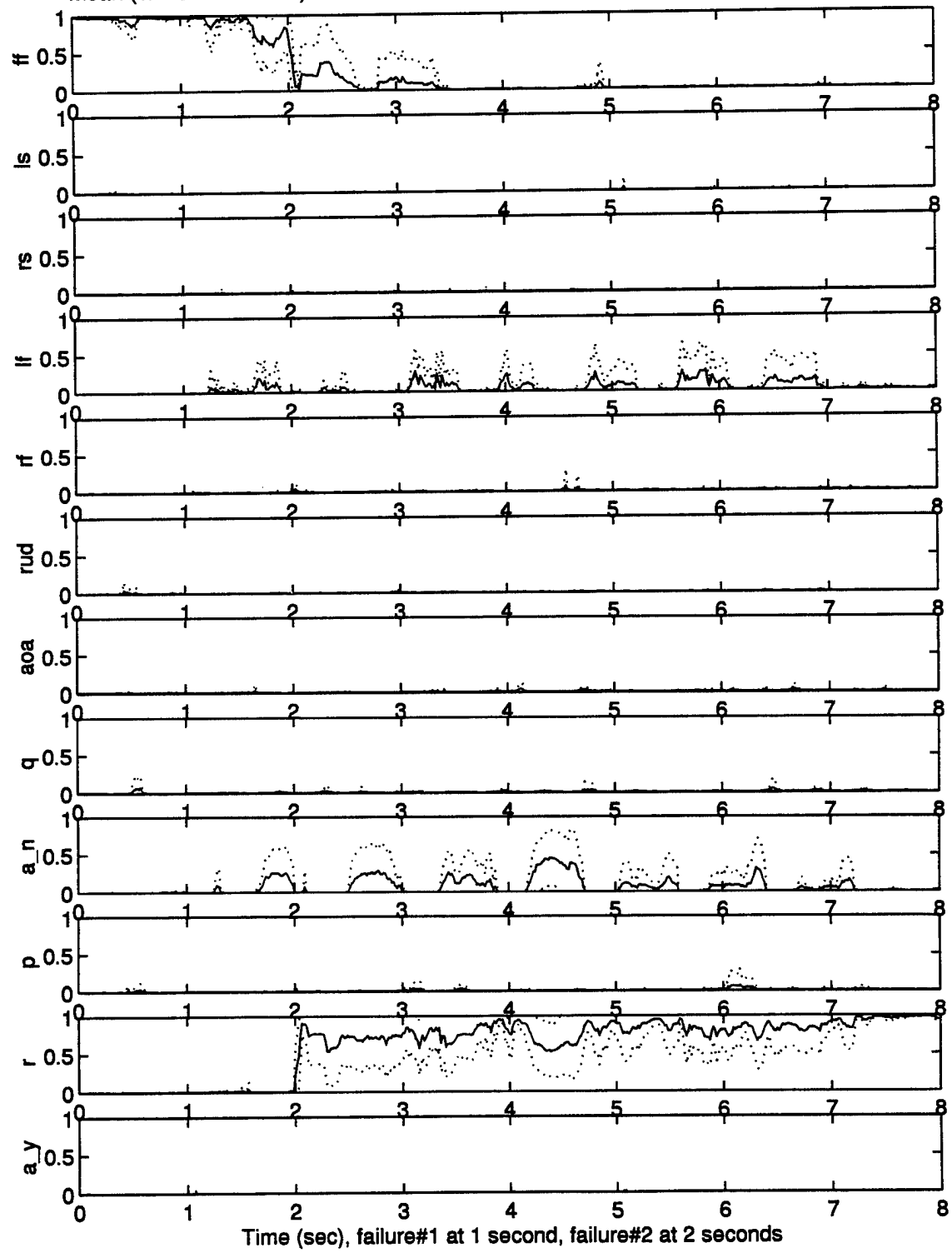
Mean (+/- One Std Dev) Dual-fail Probabilities of fail503.010 with reconfiguration: 10 runs
