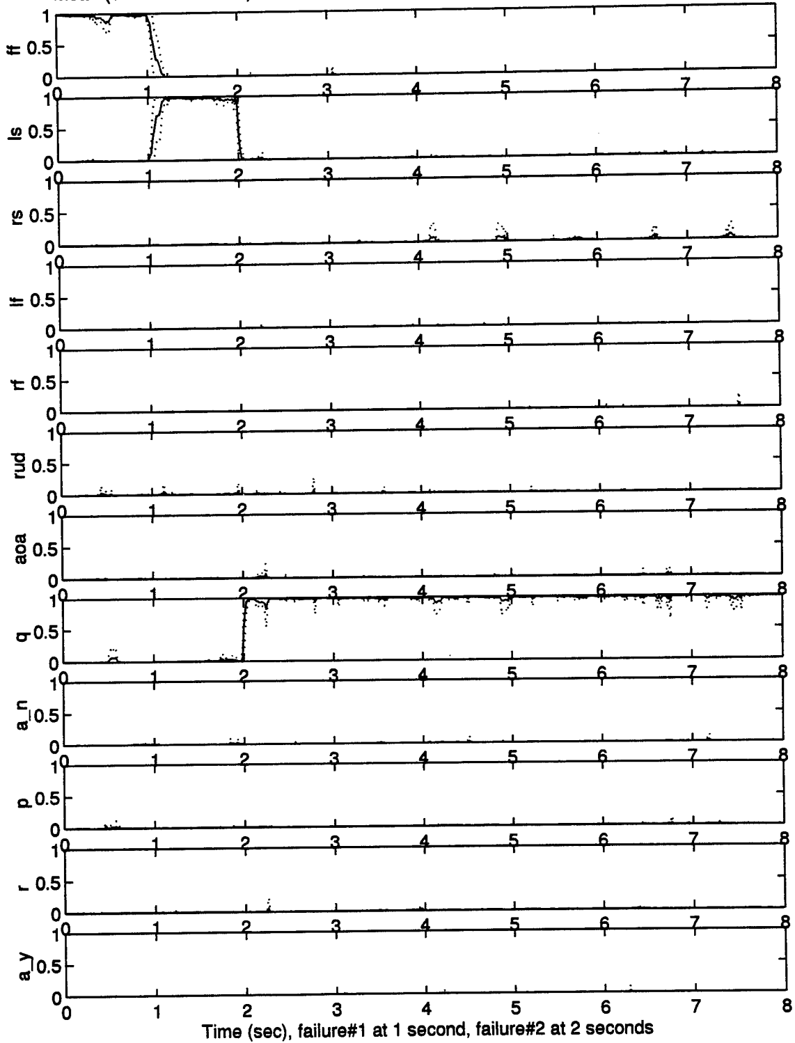
Mean (+/- One Std Dev) Dual-fail Probabilities of fail001.007 with reconfiguration: 10 runs
