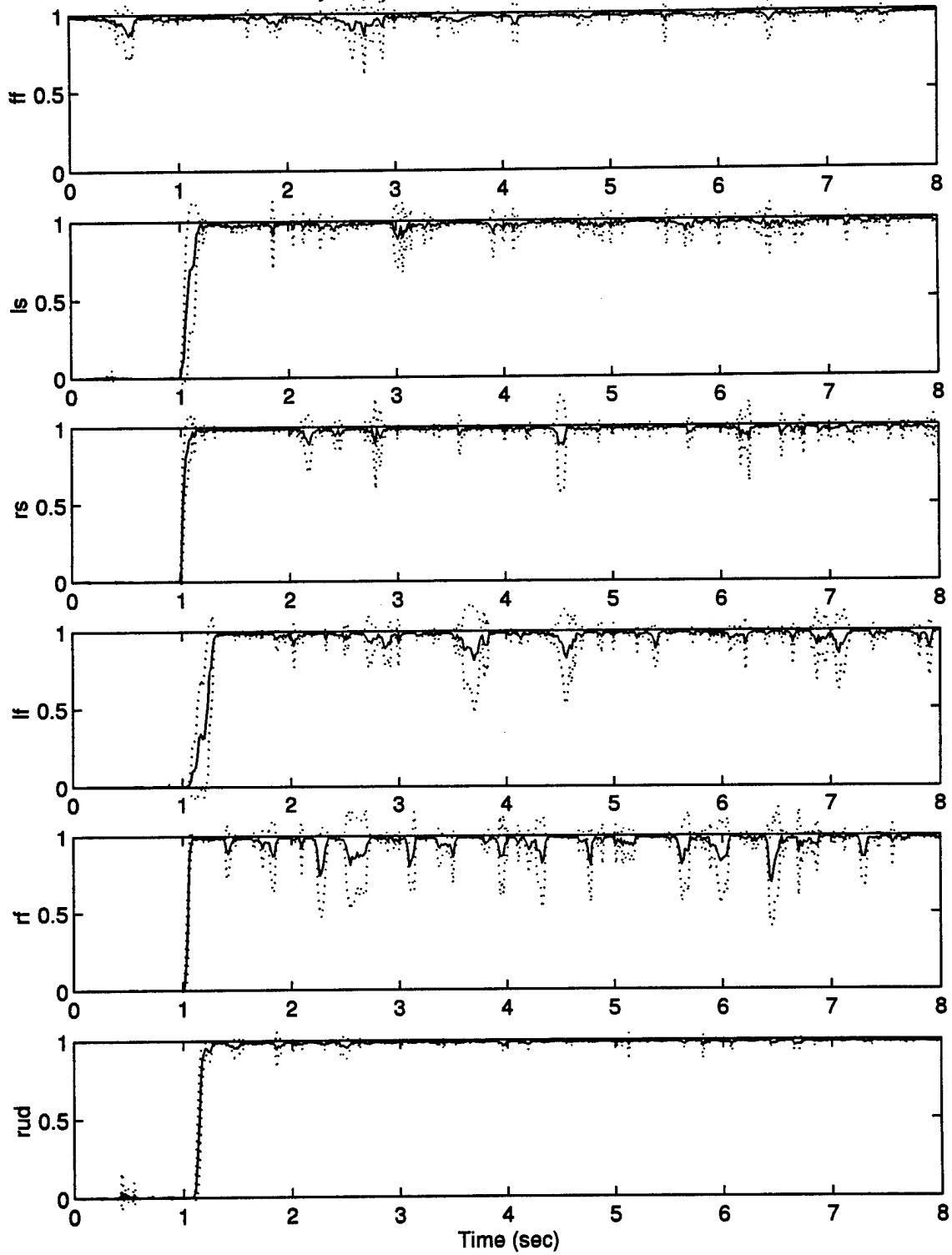
Summary Plot (with Mean +/- Sigma) for curt0: 10 runs
