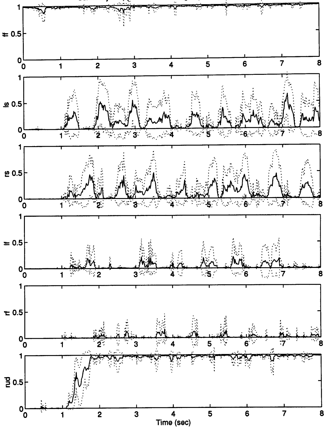
Summary Plot (with Mean \pm Sigma) for curt50: 10 runs
