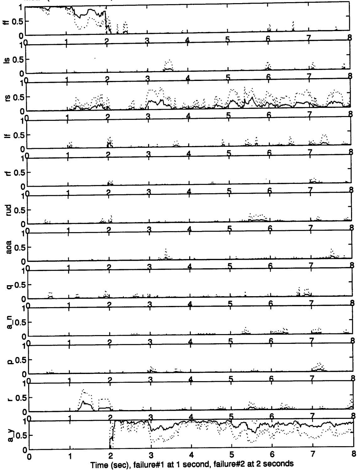
Mean (+/- One Std Dev) Dual-fail Probabilities of fail502.011 with reconfiguration: 10 runs
