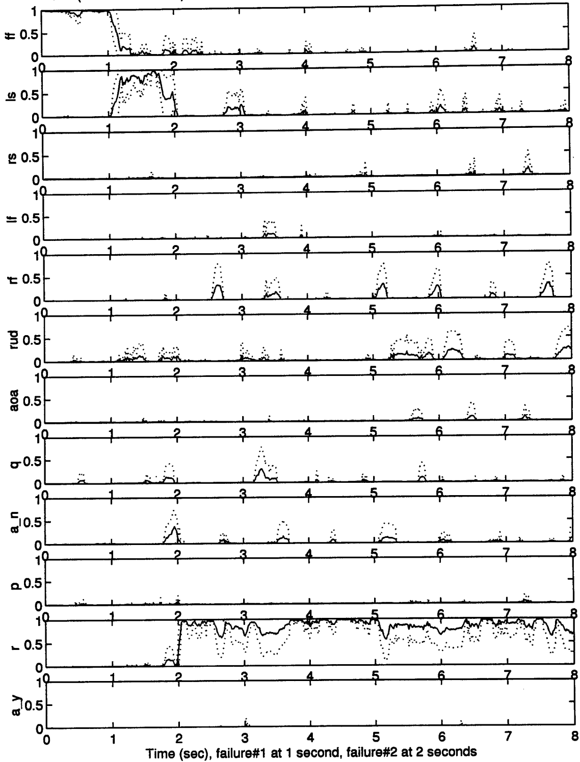
Mean (+/- One Std Dev) Dual-fail Probabilities of fail251.010 with reconfiguration: 10 runs
