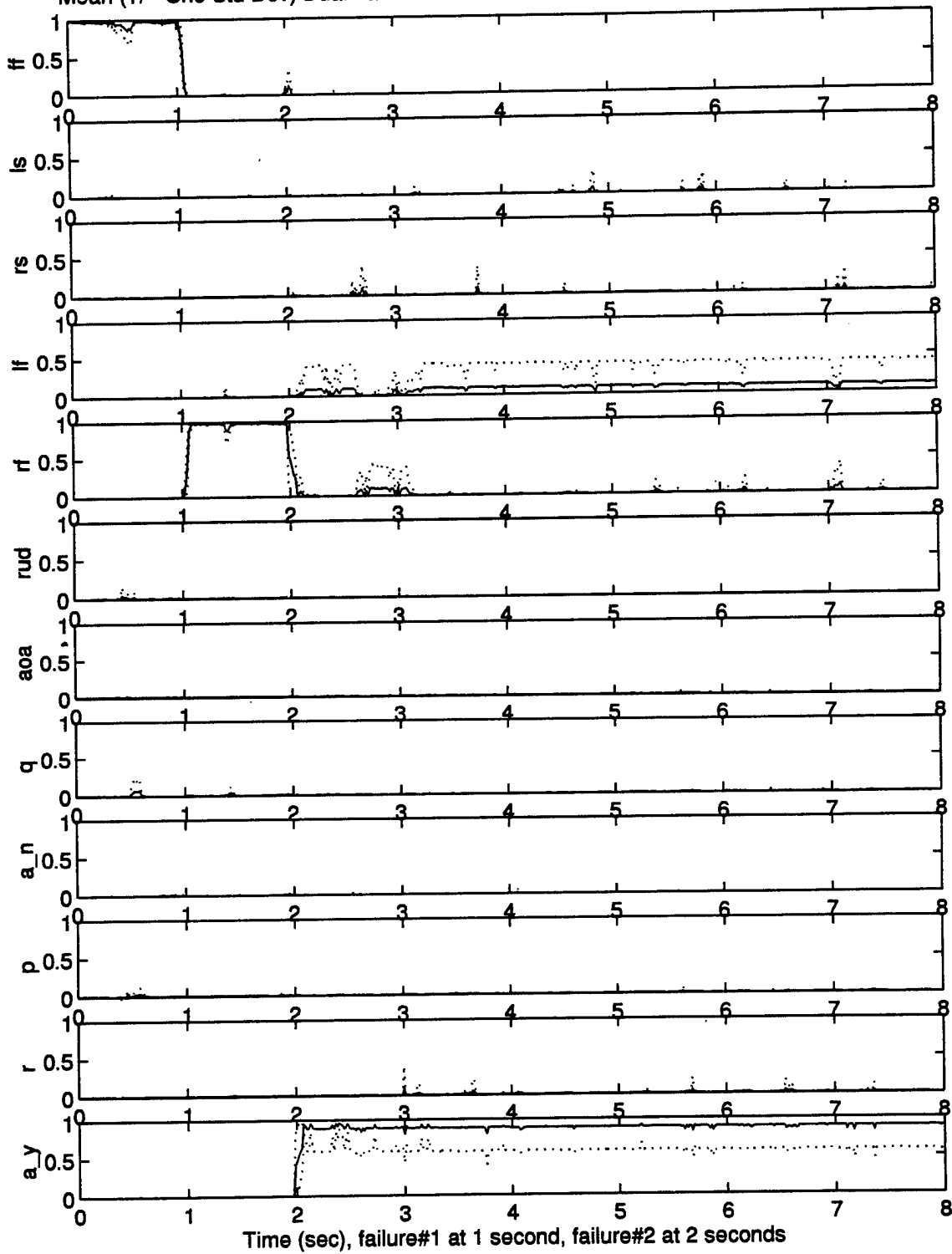
Mean (+/- One Std Dev) Dual-fail Probabilities of fail004.0011 with reconfiguration: 10 runs
