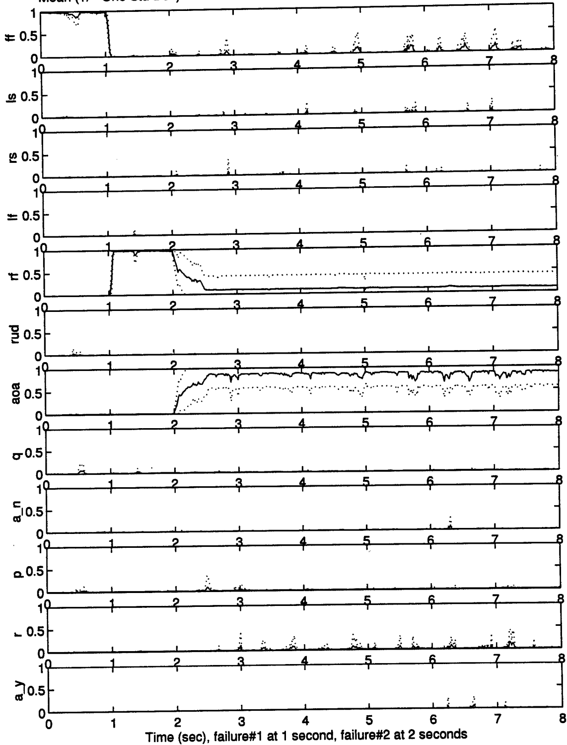
Mean (+/- One Std Dev) Dual-fail Probabilities of fail004.006 with reconfiguration: 10 runs
