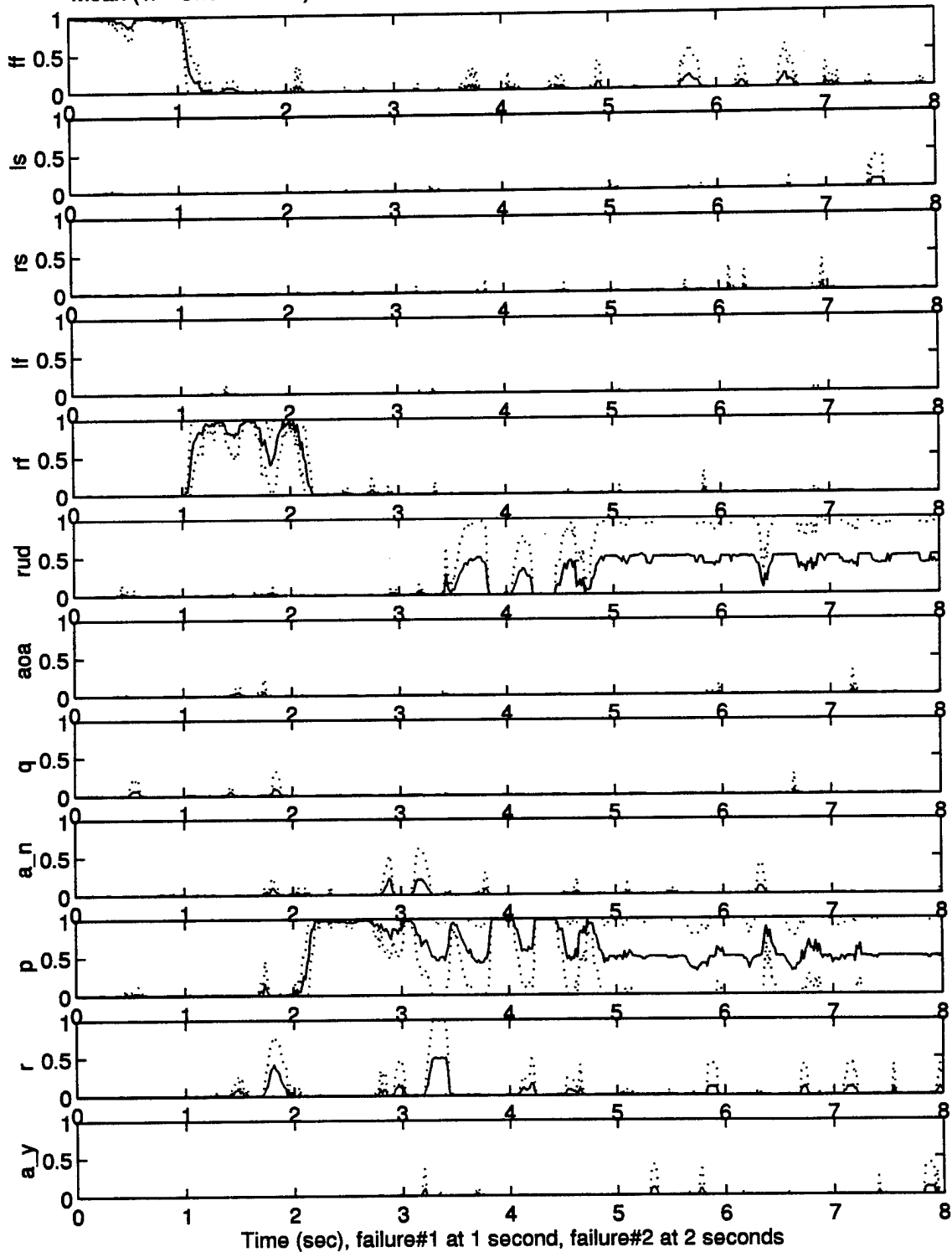
Mean (+/- One Std Dev) Dual-fail Probabilities of fail254.09 with reconfiguration: 10 runs
