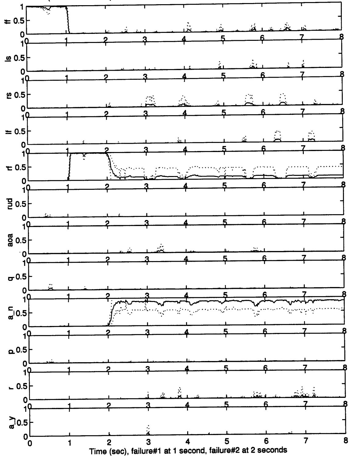
Mean (+/- One Std Dev) Dual-fail Probabilities of fail004.008 with reconfiguration: 10 runs
