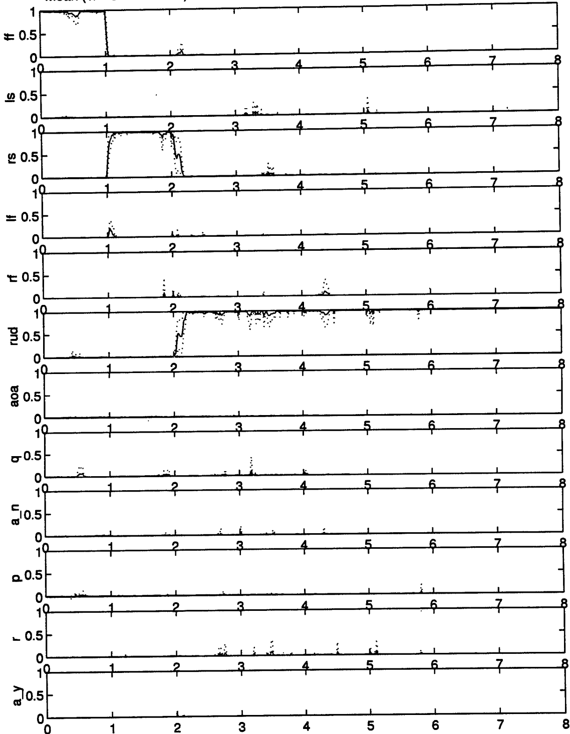
Time (sec), failure#1 at 1 second, failure#2 at 2 seconds
