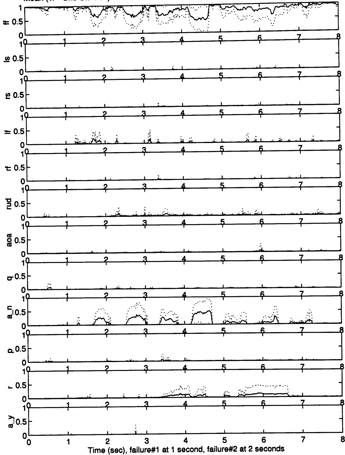
Mean (+/- One Std Dev) Dual-fail Probabilities of fail503.505 with reconfiguration: 10 runs
