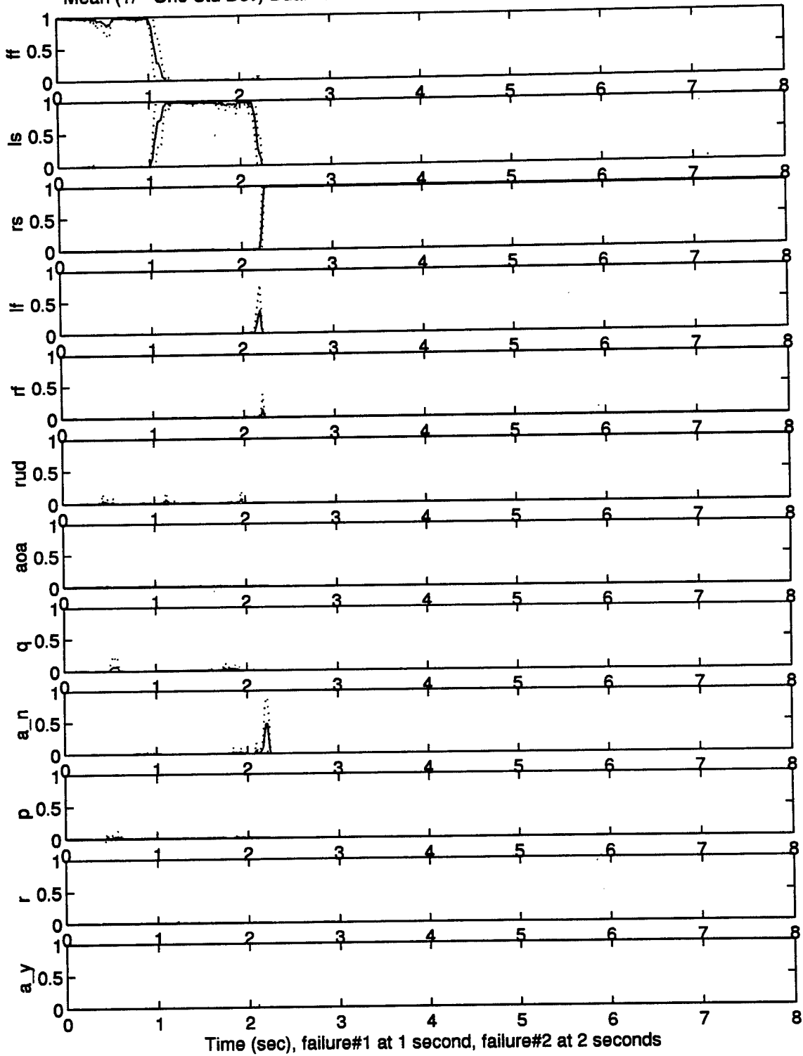
Mean (+/- One Std Dev) Dual-fail Probabilities of fail01.02 with reconfiguration: 10 runs
