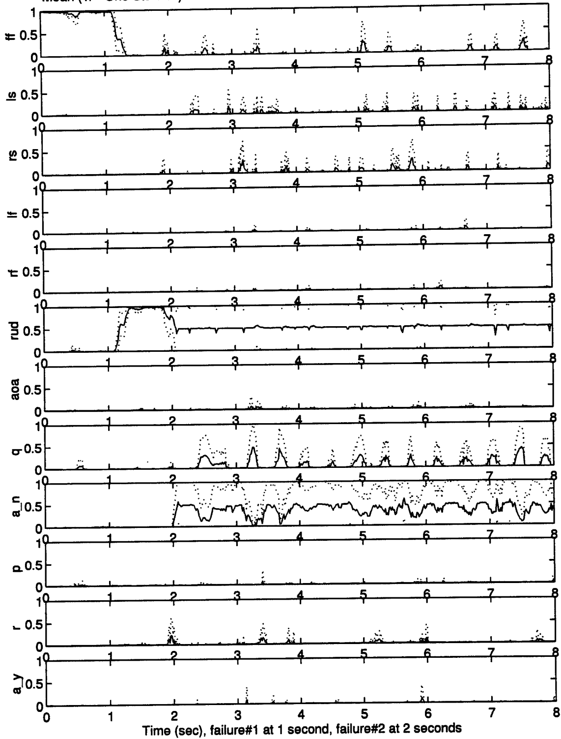
Mean (+/- One Std Dev) Dual-fail Probabilities of fail255.08 with reconfiguration: 10 runs
