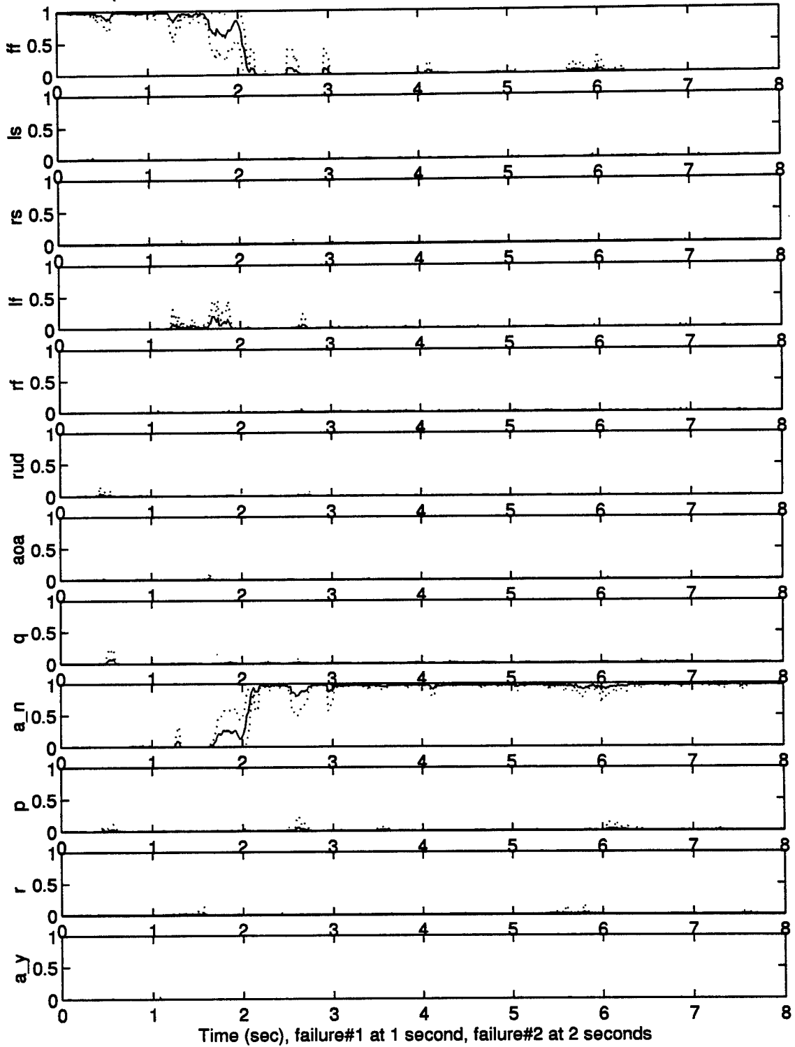
Mean (+/- One Std Dev) Dual-fail Probabilities of fail503.08 with reconfiguration: 10 runs
