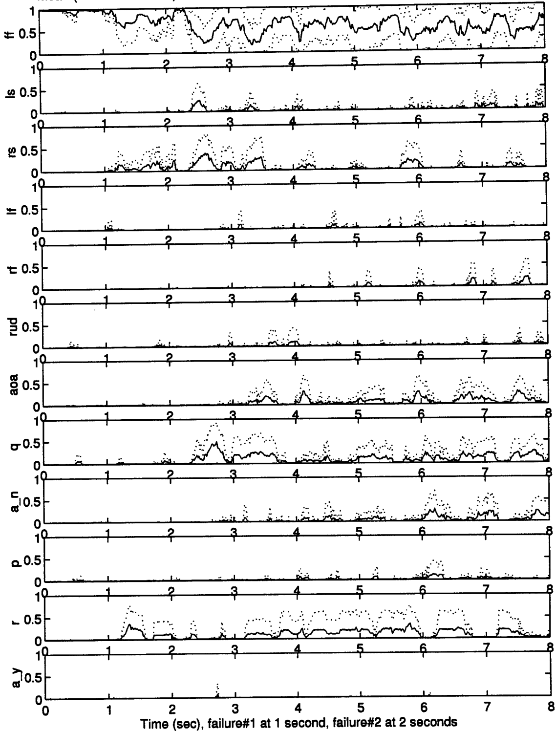
Mean (+/- One Std Dev) Dual-fail Probabilities of fail502.501 with reconfiguration: 10 runs
