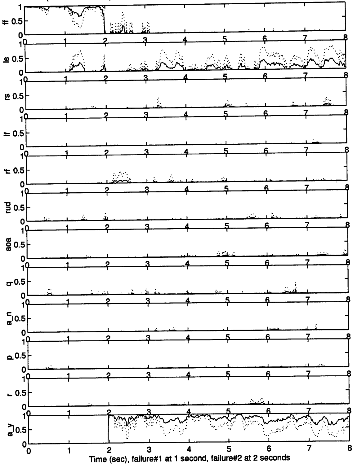
Mean (+/- One Std Dev) Dual-fail Probabilities of fail501.011 with reconfiguration: 10 runs
