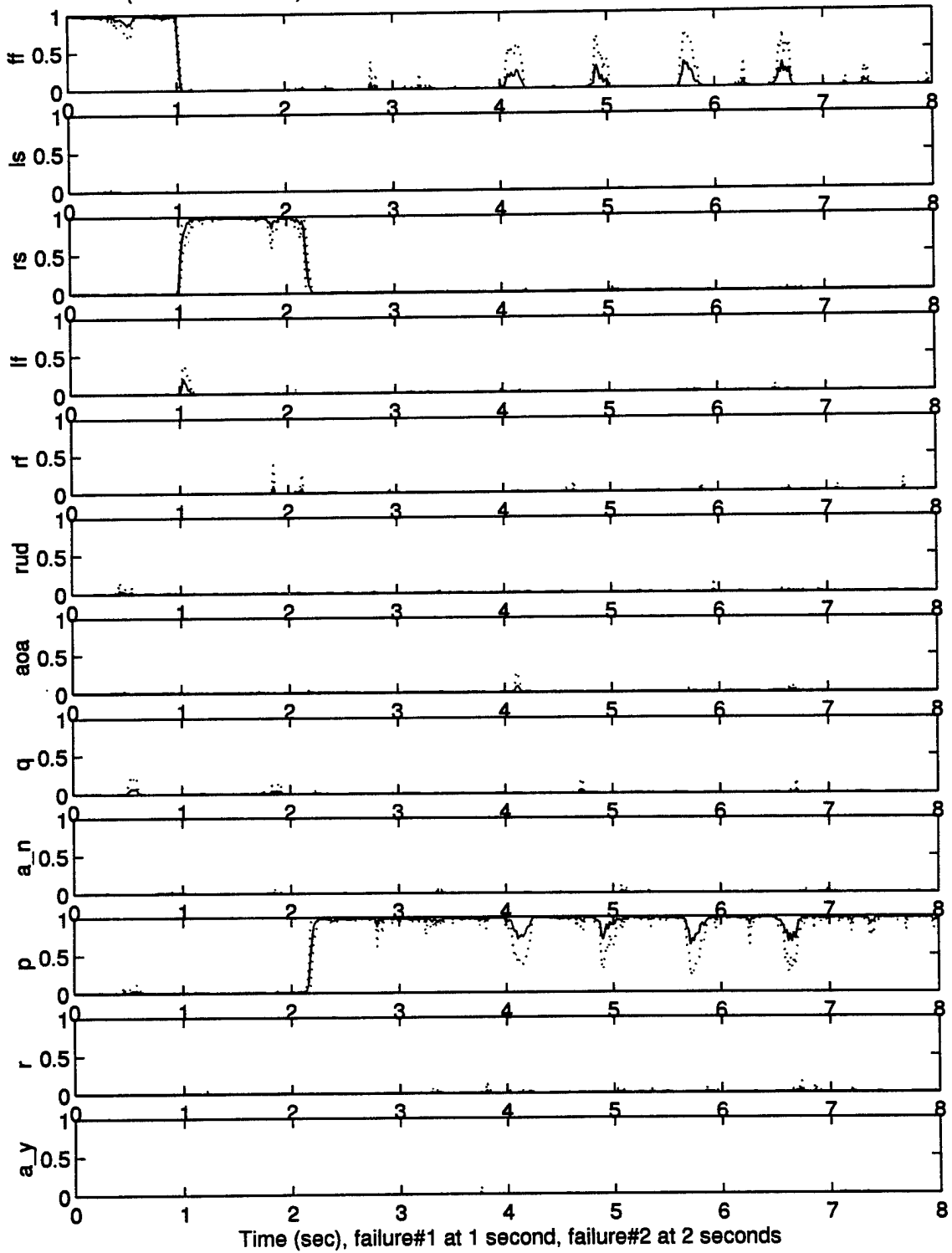
Mean (+/- One Std Dev) Dual-fail Probabilities of fail002.009 with reconfiguration: 10 runs
