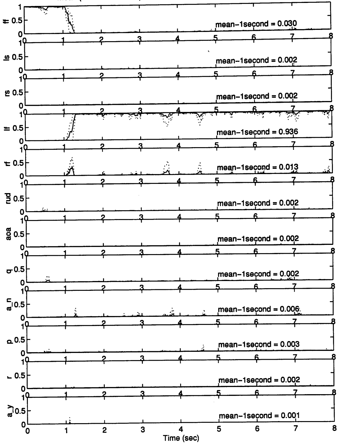
Mean (+/- One Std Dev) Probabilities of Left Flaperon Failure: 10 runs
