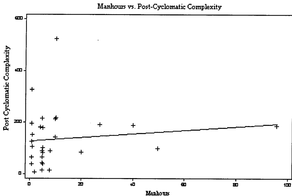
Figure H-4. Manhours vs. Post-Cyclomatic Complexity
