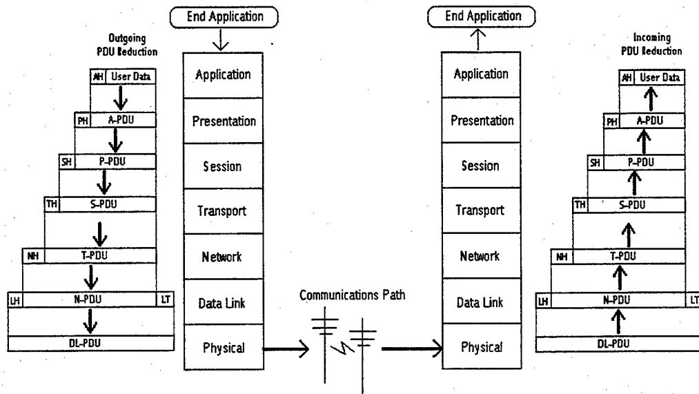
Figure 2.1 - The OSI Model [6]
