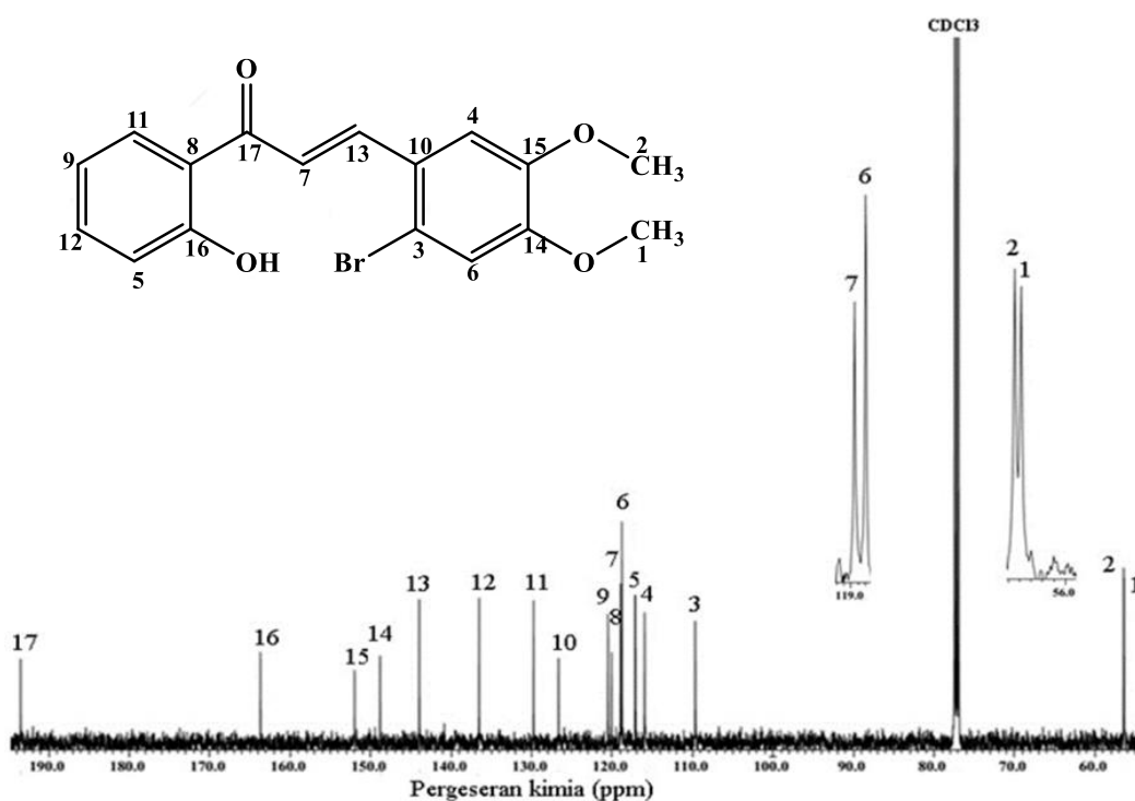
Figure 4. The ^{13}\text{C-NMR} spectra of 2'-hydroxy-2-bromo-4,5-dimethoxychalcone
