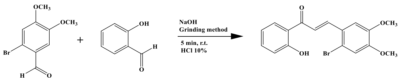
Figure 3. Synthesis of Chalcone by grinding method
