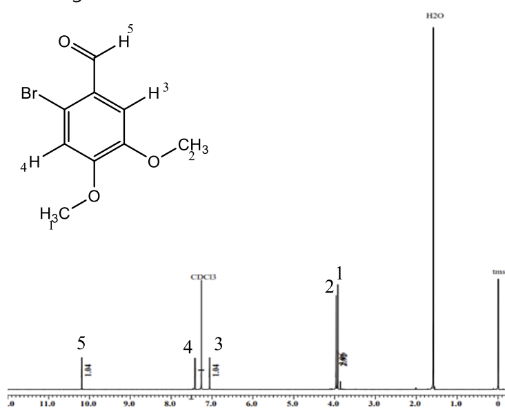
Figure 2. The spectra ^1\text{H-NMR} of 6-bromoveratraldehyde
