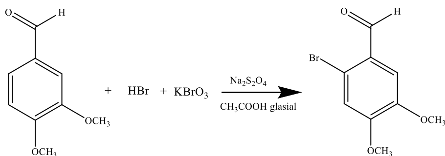
Figure 1. Synthesis 6-bromoveratraldehyde
