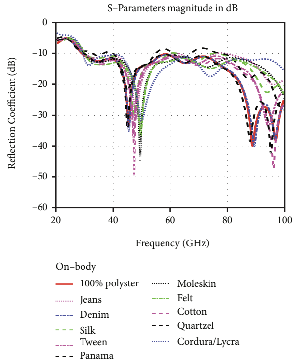
FIGURE 11: Simulated on-body return loss at different distances.
