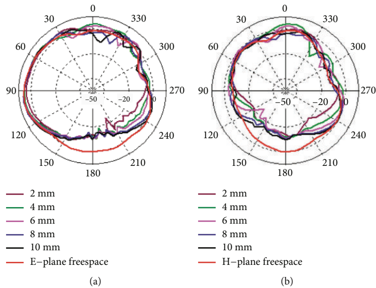
FIGURE 9: On-body radiation pattern at 60 GHz: (a) E plane and (b) H plane.
