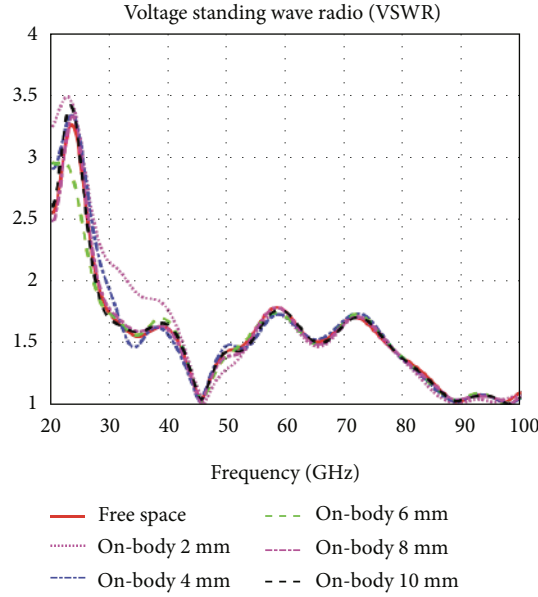
FIGURE 10: Free space and on-body (various distances) VSWR.
