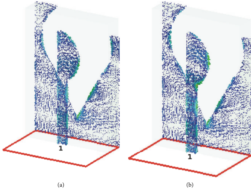
FIGURE 5: (a) Current distribution at 55 GHz and (b) current distribution at 65 GHz.
