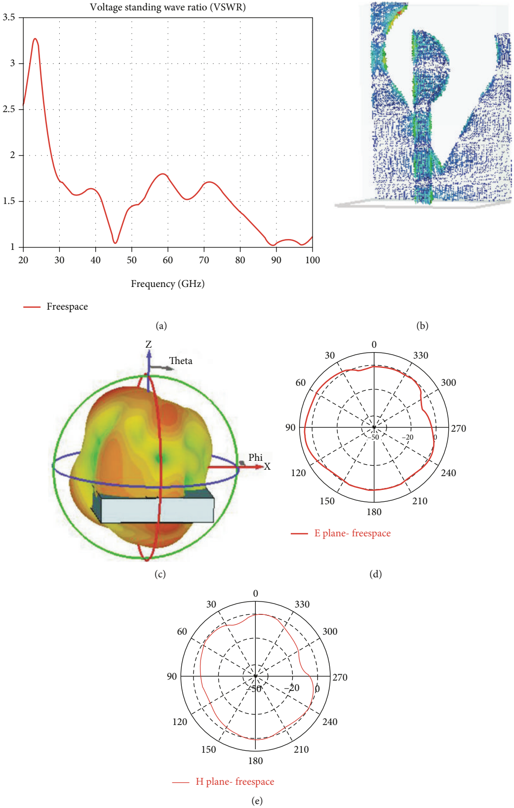
FIGURE 3: (a) VSWR, (b) surface current at 60 GHz, (c) 3D radiation pattern, (d) E plane radiation pattern at 60 GHz, and (e) H plane radiation pattern at 60 GHz.
