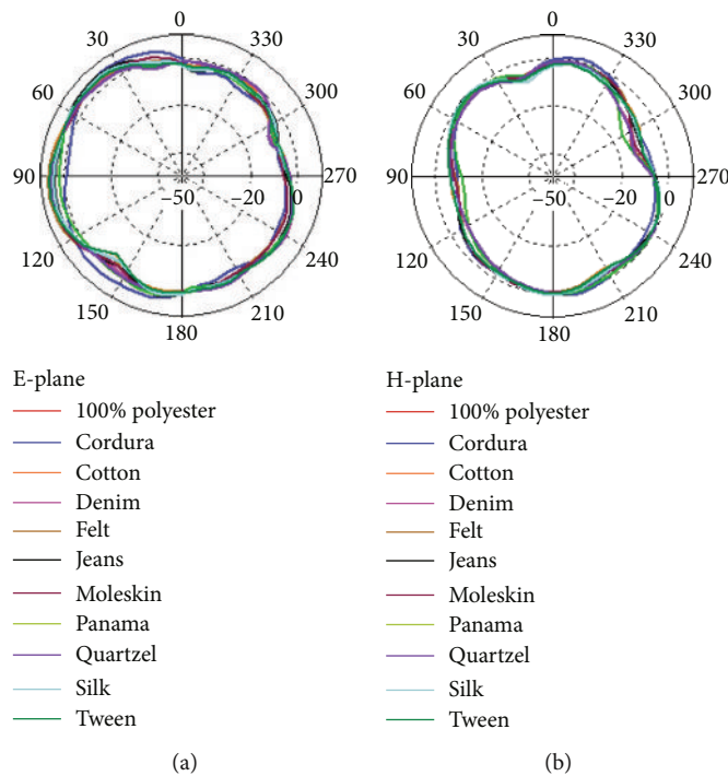
FIGURE 12: Comparison of several textile substrates' 60 GHz radiation patterns in free space: (a) E plane and (b) H plane.
