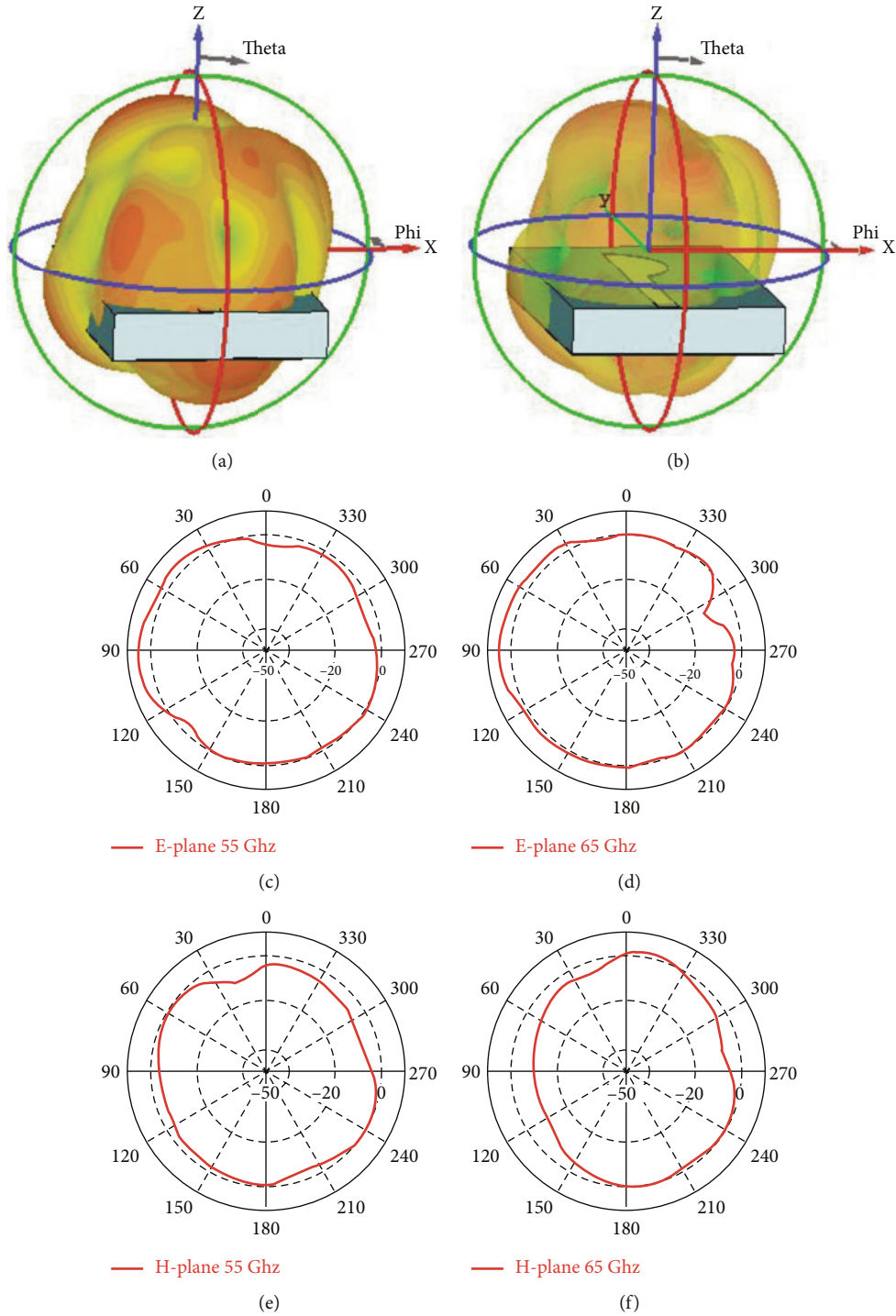
FIGURE 4: (a) 3D radiation at 55 GHz, (b) 3D radiation at 65 GHz, (c) E plane radiation at 55 GHz, (d) E plane radiation at 65 GHz, (e) H plane radiation at 55 GHz, and (f) H plane radiation at 65 GHz.
