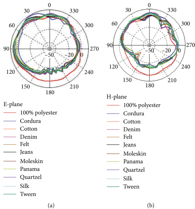
FIGURE 14: Comparison of on-body 60 GHz radiation patterns of different textile substrates: (a) E plane and (b) H plane.
