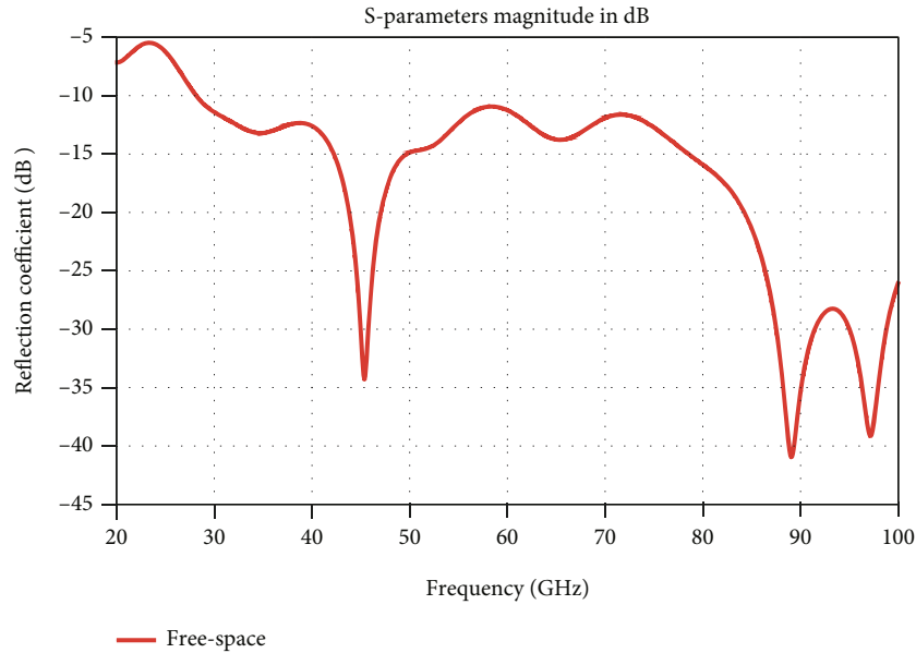
FIGURE 2: The proposed design's simulated free space return loss.
