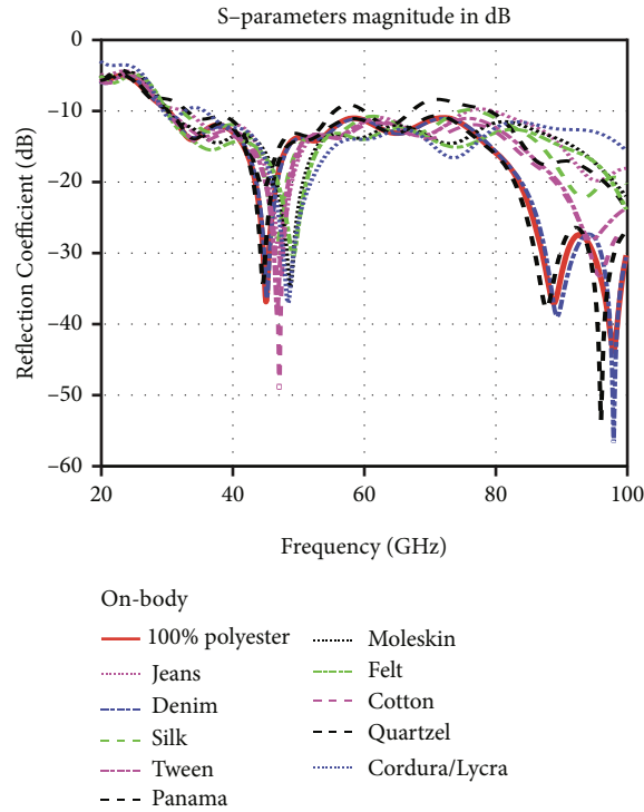
FIGURE 13: Different textile substrate on-body return losses.
