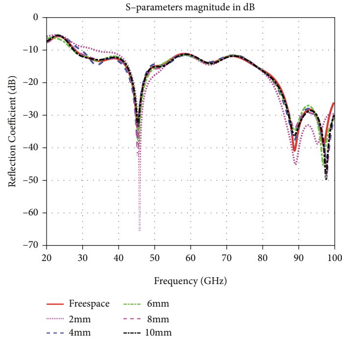
FIGURE 8: Simulations of on-body return loss at various distances.
