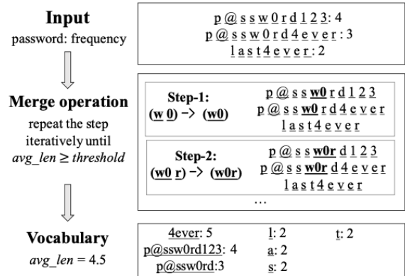
Figure 3. Example of the PwdSegment method (Taken from [8]).
