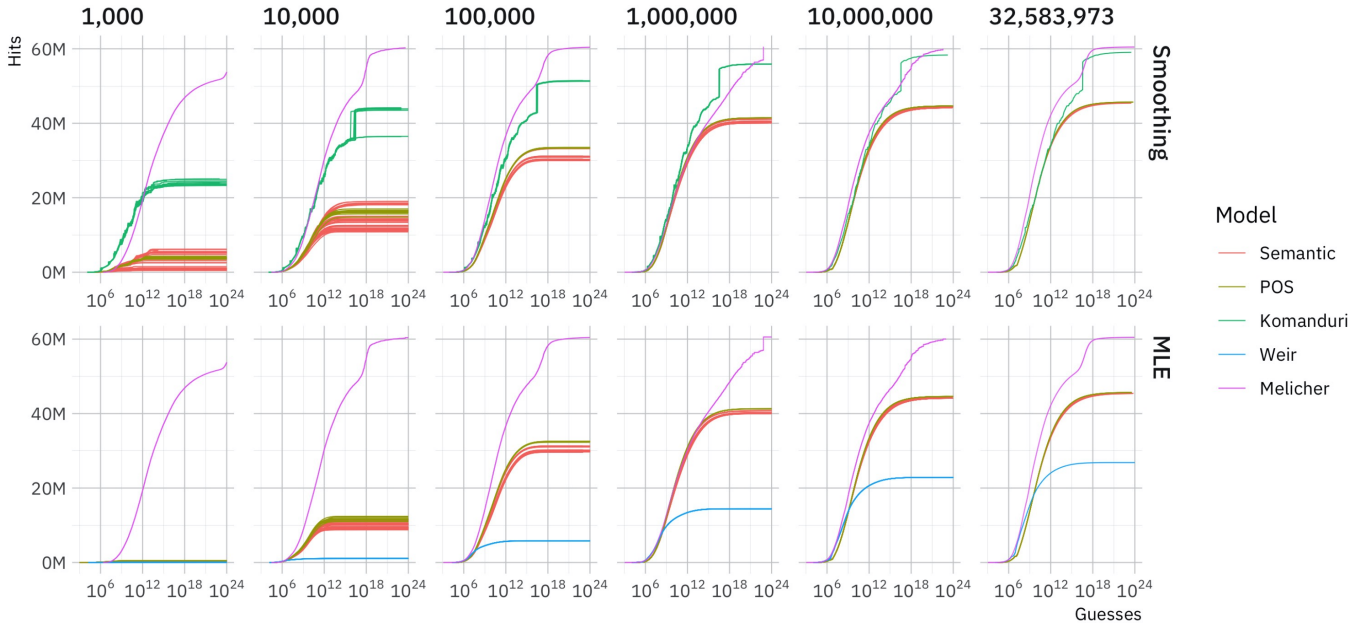
Figure 2. The results of the LinkedIn test. Each graph corresponds to the training set size as seen at the top. The total number of guesses made in each test is labeled on the horizontal axis and the number of correctly guessed passwords is on the vertical axis (Taken from [6]).
