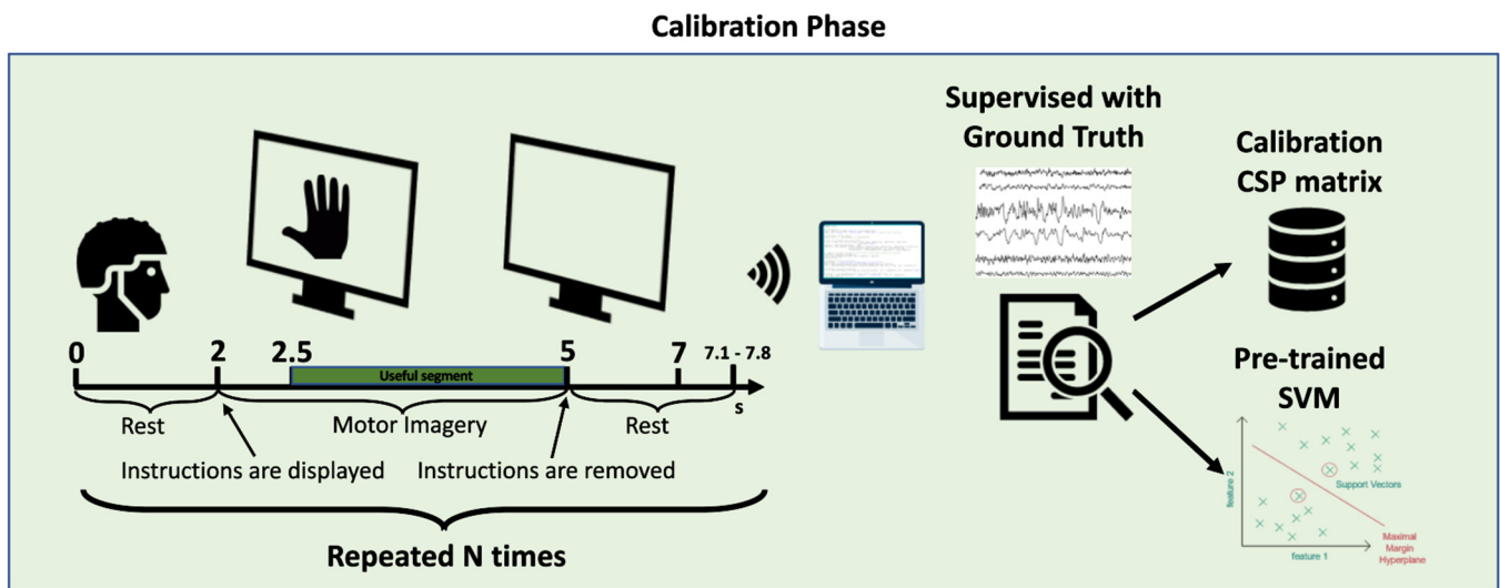
Figure 1. Calibration phase: In the calibration phase, the user watches a distant monitor, waiting for instructions. After 2 s, a left or right hand is displayed for 3 s and then removed. During this time, the user has to imagine moving their corresponding hand and then rest for 2 s. This cycle is repeated N times, with a randomic 0.1–0.8-s extension of the resting interval. Only a 2.5-s epoch of EEG signal is considered for further processing (labeled in green). Each trial, along with its ground truth label (right/left), is used to construct the calibration CSP matrix from which a set of features is extracted and used to train an SVM classifier.
