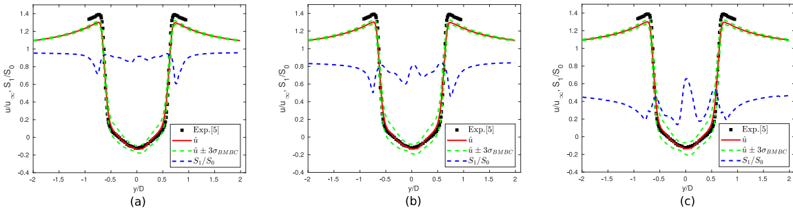
FIGURE 3. Study on the batch size effect with \Delta t = 0.25 (a), 0.5 (b) and 1(c) convective times.
