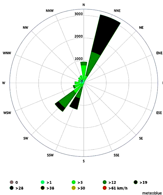
Fig. 4. Wind direction in Industrial Park Arequipa (Meteoblue, 2019)
