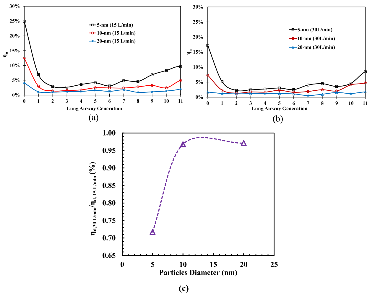
Fig. 10. Particle deposition efficiency in airway lung generation: (a) Q_{in} = 15 L/min; (b) Q_{in} = 30 L/min; (c) Ratio of the deposition rates at the two flow rates.
