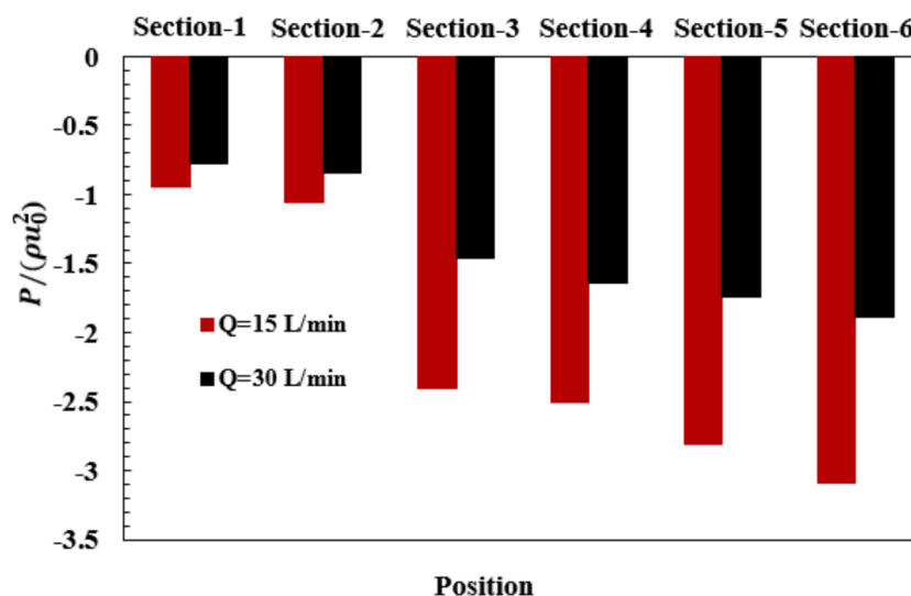
Fig. 9. Pressure drop at two distinct flow rates in a different section of the lung model; the section numbers are shown in Fig. 1.
