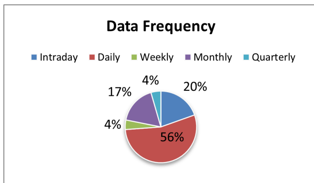
Figure 3: Surveyed papers grouped by Sampling frequency.
