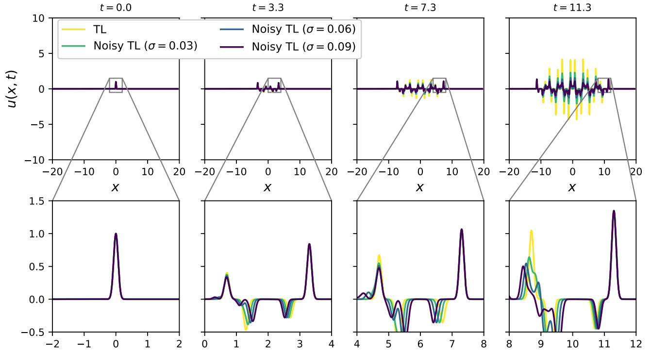
Figure 13: Snapshots of the amplitude of a Gaussian pulse of the form u(x, 0) = \exp(-100x^2) , as it propagates through a time laminate, with \alpha_1 = \beta_1 = 1 , \alpha_2 = \beta_2 = 0.5 , and the period of time modulation T = 1 , with various degrees of disorder.
