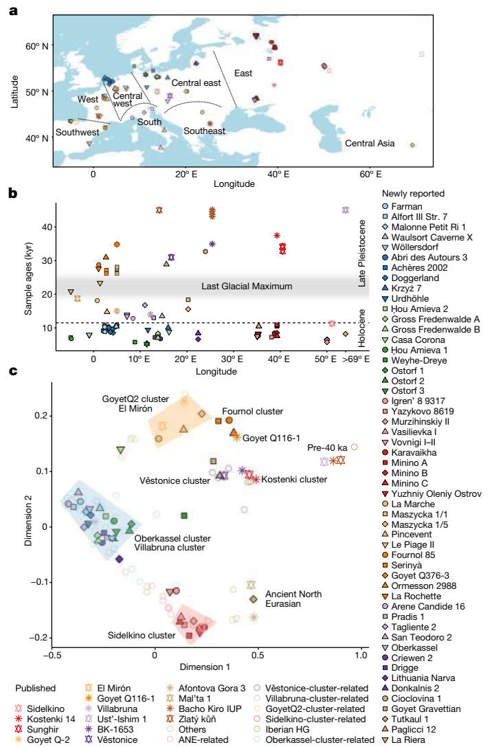
Fig. 1 | Locations, dates and MDS plot of ancient Eurasian hunter-gatherers. a , Geographic locations of newly reported individuals (filled symbols with black outline) and representative previously published individuals (outlined stars). Dotted lines delimit geographic regions described in the text. b , Calibrated radiocarbon dates of individuals plotted in a . The y-axis shows the average of calibrated radiocarbon dates in thousands of years (kyr) (Supplementary Data 1.A). The horizontal dashed line marks the boundary between Late Pleistocene and Holocene. c , MDS plot of European hunter-gatherers based on 1 - f_3(\text{Mbut}; \text{pop1}, \text{pop2}) . The dimensions are calculated using newly reported and previously published hunter-gatherer groups or individuals with more than 30,000 SNPs. The detailed grouping of individuals shown with empty coloured circles is described in Supplementary Data 1.I.
