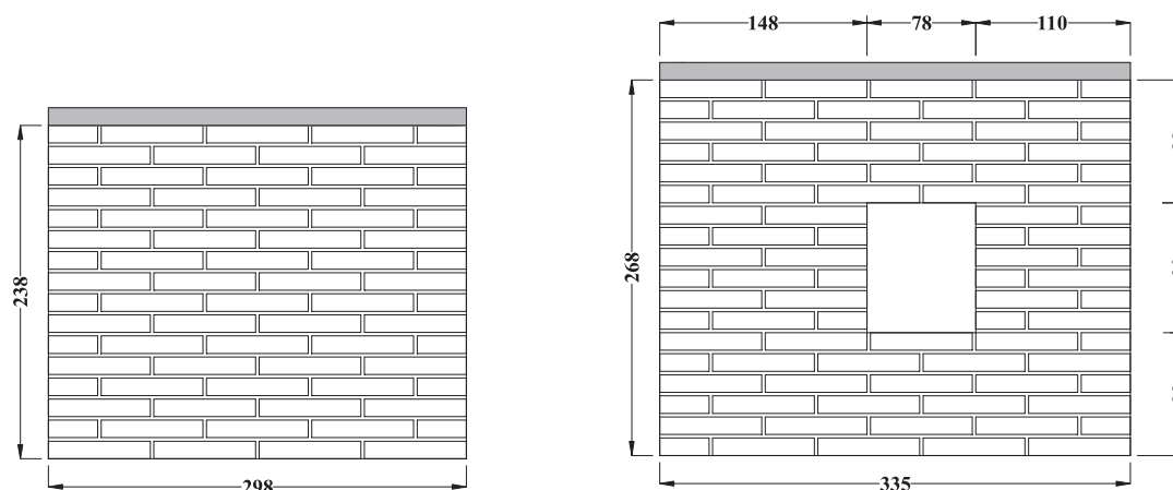
Fig. 8. Geometry of tested masonry solid and perforated walls. Dimensions in mm.
