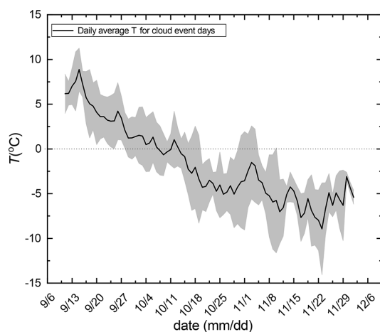
Figure 5. The daily average temperatures at the Sammaltunturi site for days with cloud events during all PaCE campaigns. The dotted line is used as a reference line for 0°C temperature. The definition of a cloud event is provided in the text. The shaded area represents the corresponding standard deviations.
