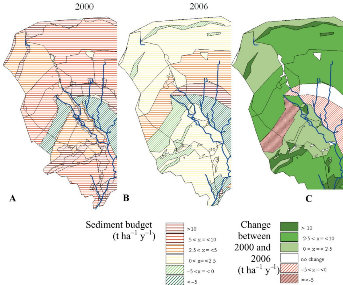
Figure 8. Sediment budget (sediment production minus sediment deposition = sediment yield) (t ha -1 y -1 ) for each land unit in 2000 (A) and 2006 (B). Sediment delivery areas (sources) are positive (red) and sediment deposition areas (sinks) are negative (green). (C): changes between 2000 and 2006 with improvements (green) and declines (red), related to decreased sediment input. Gully erosion and deposition behind check dams are not represented.
