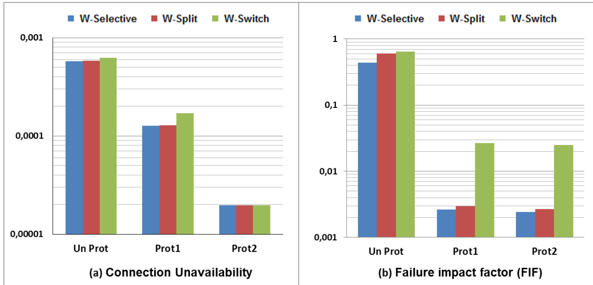
Figure 4: Connection unavailability (a) and FIF (b) for various HPON architectures.
