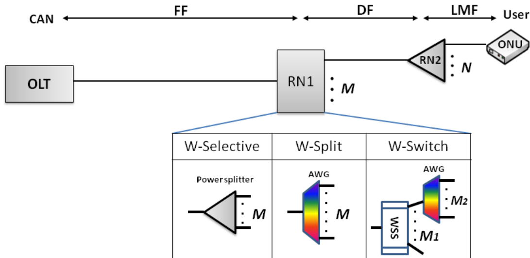
Figure 1: Basic HPON architecture with different options for RN1.
