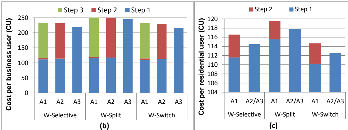
Figure 5: (a) Detailed CAPEX per user considering A3, cost per (b) Business user and (c) Residential user for HPON architectures considering three protection upgrade approaches
