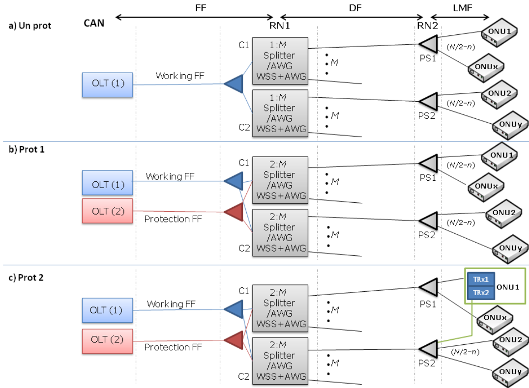
Figure 2: HPON (a) without protection, (b) with protection up to RN1 for all connected ONUs and (c) E-to-E protection for some selected ONUs compatible with all HPON variants.
