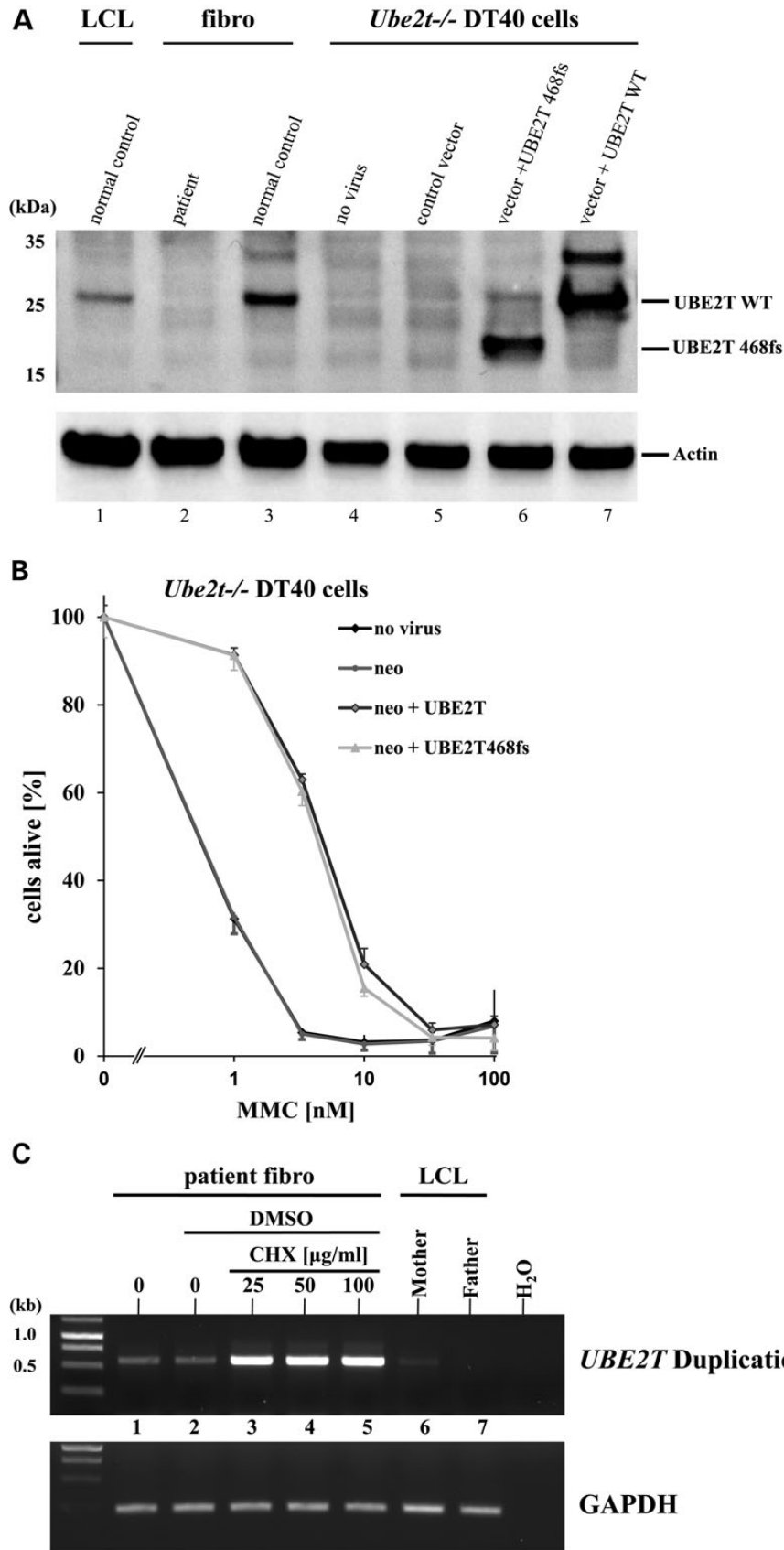
Figure 3. Functional analysis of the mutations and NMD. (A) Expression of the mutant UBE2T 468fs protein in Ube2t -/- DT40 cells. Cell lysates from a normal B-cell line (LCL), immortalized patient and normal control fibroblasts, non-transduced DT40 cells (no virus), and DT40 cells transduced with the control, UBE2T 468fs or WT UBE2T
