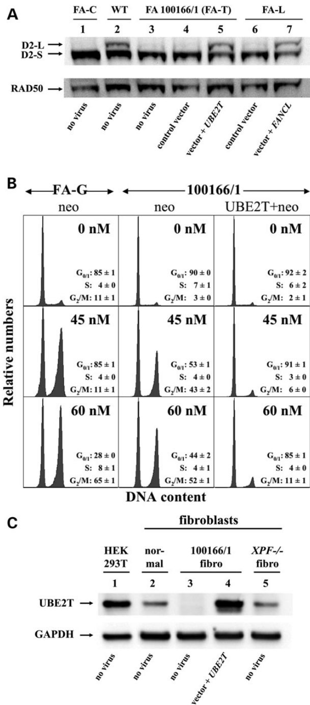
Figure 1. Identification of UBE2T as new FA gene by retroviral complementation of FA 100166/1 fibroblasts and western blotting. (A) Western blot analysis of protein extracts from transduced fibroblast lines immunostained with a FANCD2 antibody to detect non-ubiquitinated (D2-S) and monoubiquitinated (D2-L) FANCD2. Lanes 1–3 depict the FANCD2 ubiquitination status of FANCC-deficient (FA-C), wild-type (WT) and FA100166/1 fibroblasts exposed to 150 nM MMC overnight. Lanes 4–7 show the FANCD2 monoubiquitination status of G418-resistant FA 100166/1 and FANCL-deficient fibroblasts, genetically modified with a control vector or with vectors expressing UBE2T or FANCL cDNAs, respectively. Staining with a RAD50 antibody was used to visually confirm equal loading. (B) Flow cytometric cell cycle analysis of transduced primary fibroblasts grown for 3 days in 0, 45 or 60 nM MMC. FA-G: primary FANCG -/- fibroblasts (38) transduced with the control vector (neo control). FA 100166/1: primary patient fibroblasts transduced with the control vector (neo control) or the UBE2T -coexpressing vector ( UBE2T + neo). The distribution of cells in G 0 /G 1 , S and G 2 /M arrest from three different experiments is shown. (C) Western blot analysis of
