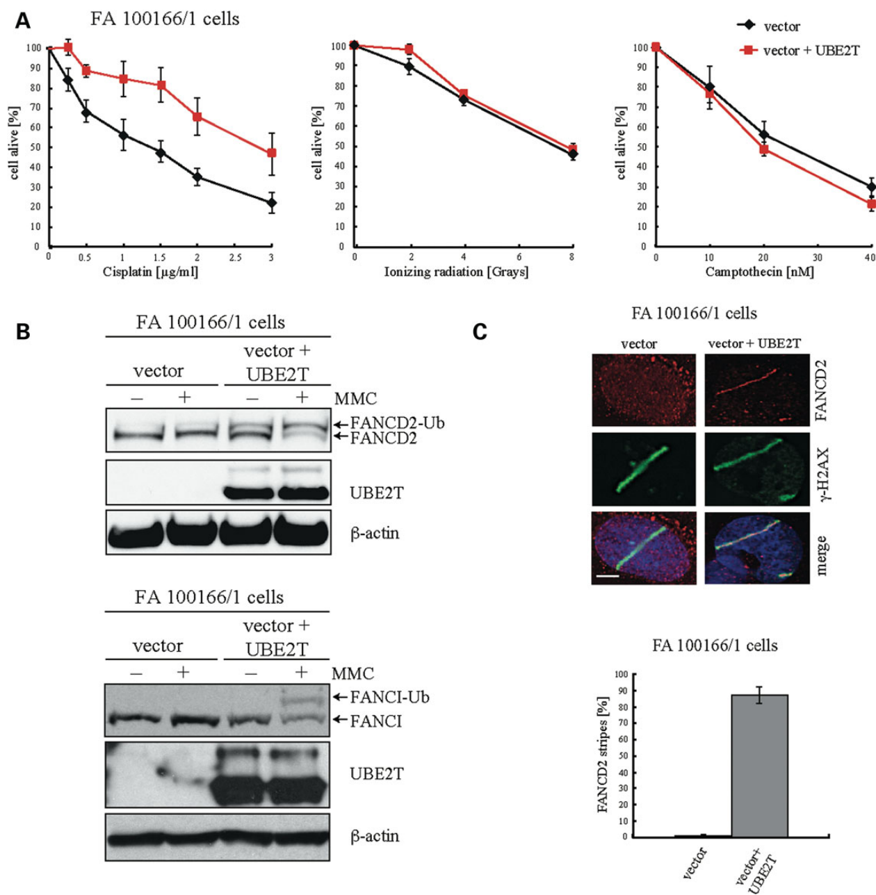
Figure 4. The cellular phenotype of human UBE2T -/- fibroblasts is comparable to that of FA cells with defects in FA core complex members. (A) Survival of UBE2T -/- fibroblasts after exposure to genotoxins. An isogenic pair of UBE2T -/- fibroblasts transduced with a retroviral vector encoding UBE2T or the corresponding control vector were exposed to increasing doses of the genotoxins cisplatin, ionizing radiation and camptothecin. (B) Western blot analysis to visualize intact FANCD2 and FANCI monoubiquitination in immortalized UBE2T -/- fibroblasts after exposure to MMC by UBE2T expression. (C) Restoration of FANCD2 recruitment to sites of DNA crosslinks by UBE2T expression. Psoralen interstrand crosslinks were induced along the track of a UVA laser in corrected and non-corrected UBE2T -/- fibroblasts and then visualized by \gamma -H2AX staining. FANCD2 accumulation at the sites of psoralen laser tracks only occurred in FA100166/1 cells that had been transduced with the UBE2T expressing retroviral vector.
