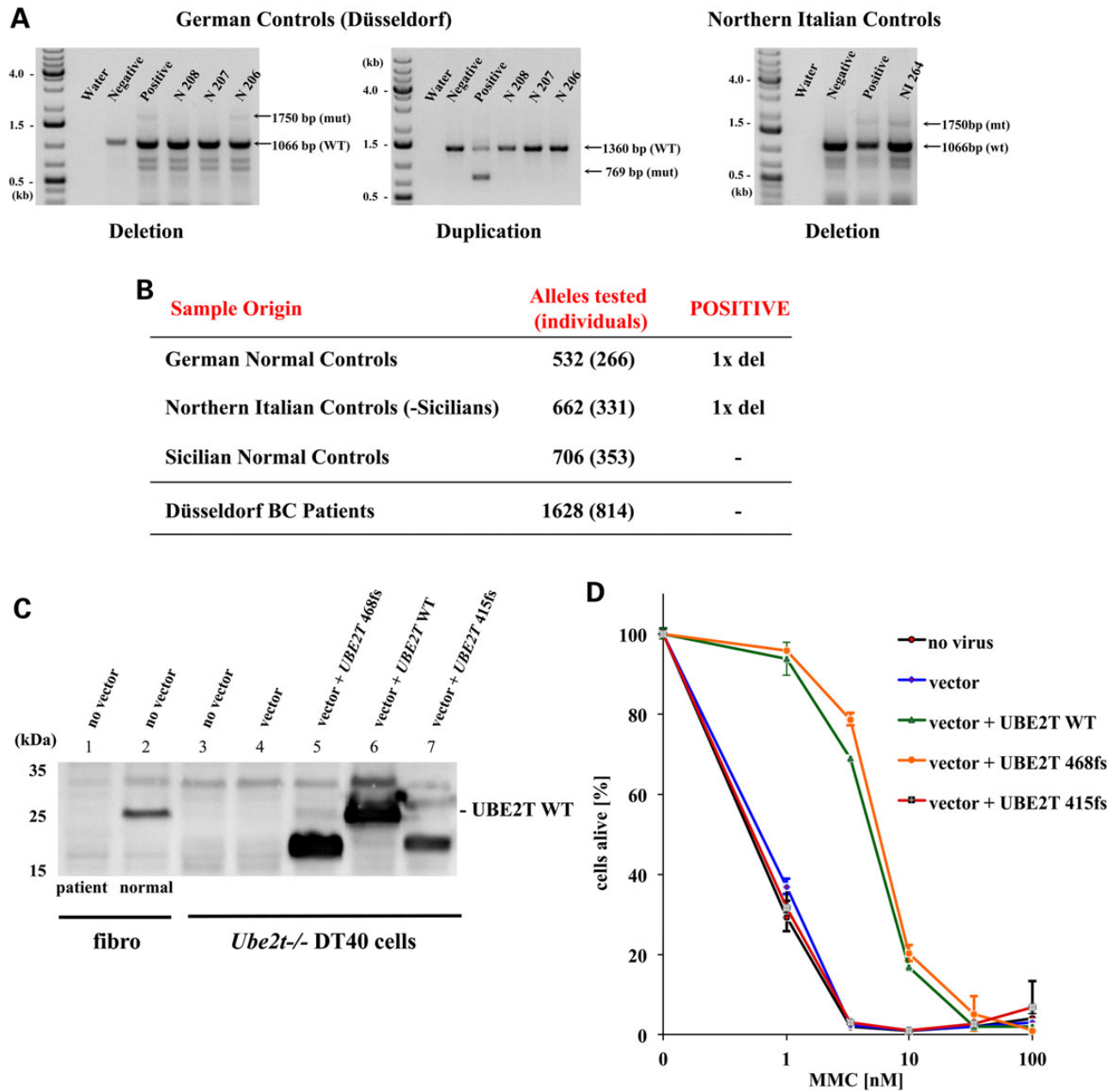
Figure 5. UBE2T mutations in normal individuals from Germany and Italy and in BRCA1/2 WT breast cancer patients. (A) Detection of the UBE2T exons 2–6 deletion in two healthy individuals. PCR analysis with primers for coamplification of the normal and mutant alleles with the exons 2–6 deletion were used to identify the deletion in genomic DNA of two normal controls, N 206 from Germany and NI 264 from Northern Italy. (B) Frequencies of the UBE2T exons 2–6 deletion and duplication in normal individuals and German breast cancer patients. The PCRs with primers for co-amplification of the normal and two mutant alleles with the exons 2–6 deletion and duplication were performed on genomic DNA from 850 normal control individuals from Germany and Italy. PCR analysis was also performed on genomic DNA of 814 breast cancer patients from the University of Düsseldorf breast cancer clinic. (C) The mutant UBE2T 415fs protein is stably expressed in Ube2t -/- DT40 cells. Cell lysates from the FA 100166/1 patient fibroblasts and normal control fibroblasts, non-transduced Ube2t -/- DT40 cells (no vector) and Ube2t -/- DT40 cells transduced with the control vector (vector), the WT UBE2T (UBE2T WT), the frameshift mutant UBE2T 468fs, or the frameshift mutant UBE2T 415fs vectors were immunoblotted and probed with the polyclonal UBE2T antibody. (D) Expression of the mutant UBE2T 415fs protein does not correct the MMC hypersensitivity of Ube2t -/- DT40 cells. Expression of the human UBE2T WT (blue line) and 468fs protein (green) increased the survival rates of Ube2t -/- DT40 chicken cells during culture with increasing concentrations of MMC for 3 days. The UBE2T 415fs mutant protein (red) did not confer any survival advantage relative to that of non-transduced (no virus, black line) and control vector-transduced (vector, blue) cells.
