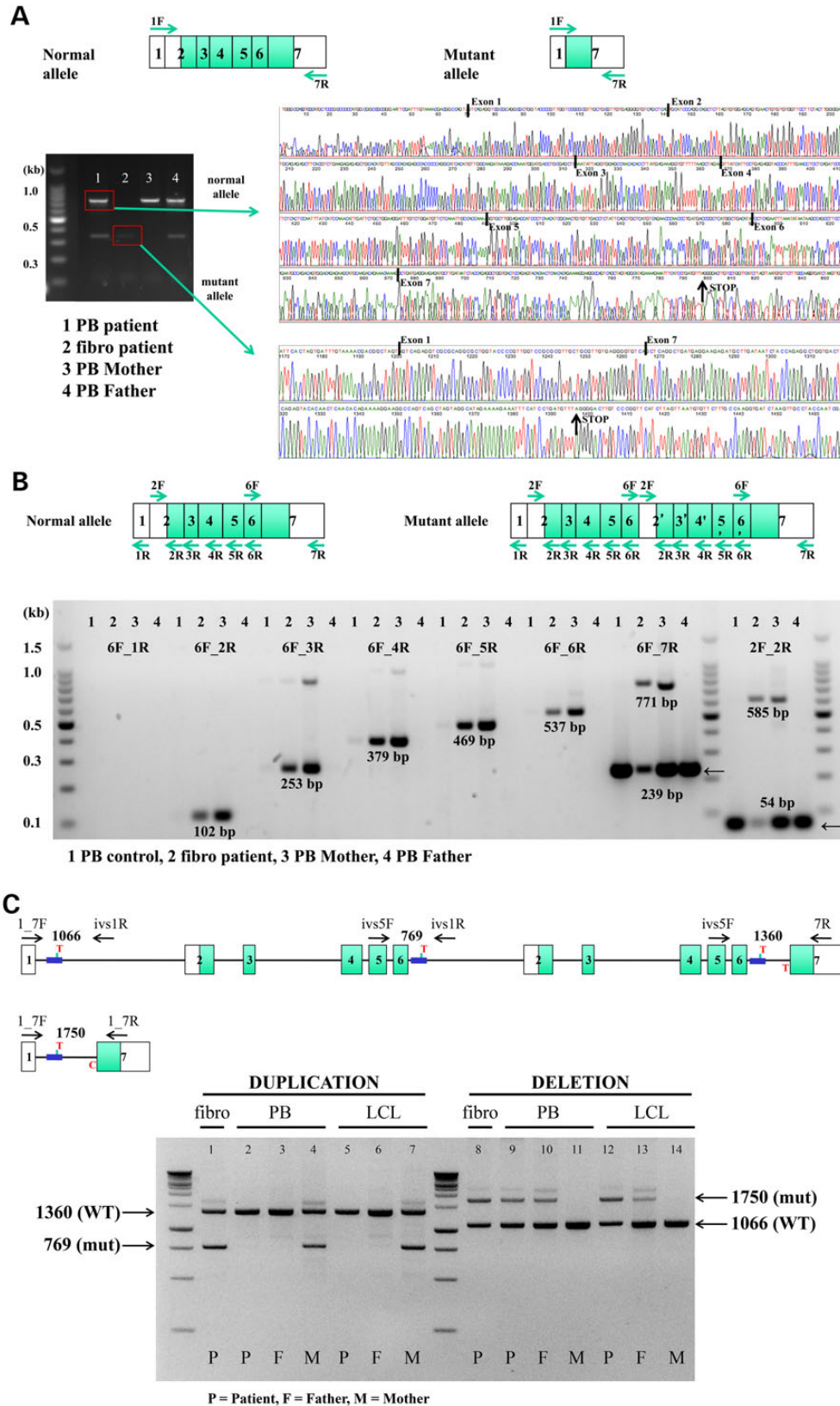
Figure 2. Identification of two aluY-mediated germline mutations in UBE2T in FA 100166/1. (A) Identification of the paternal exons 2–6 deletion in UBE2T in cDNA. Forward and reverse primers in exons 1 (1F) and 7 (7R) were utilized in cDNA from the peripheral blood (PB) and fibroblasts (fibro) of the FA 100166/1 patient. The PB from the patient was sampled at 14 years of age. cDNA was also obtained from the PB of the mother (PB Mother) and father (PB Father). The amplified PCR products were run on a gel, and the bands excised and sequenced. Sequencing traces for two of the bands are shown. Boundaries of the different exons are indicated. (B) Identification of the maternal exons 2–6 duplication in UBE2T in cDNA. cDNA was generated from the primary fibroblasts of the patient (Fibro patient) and the PB of a normal individual (PB control), the mother
