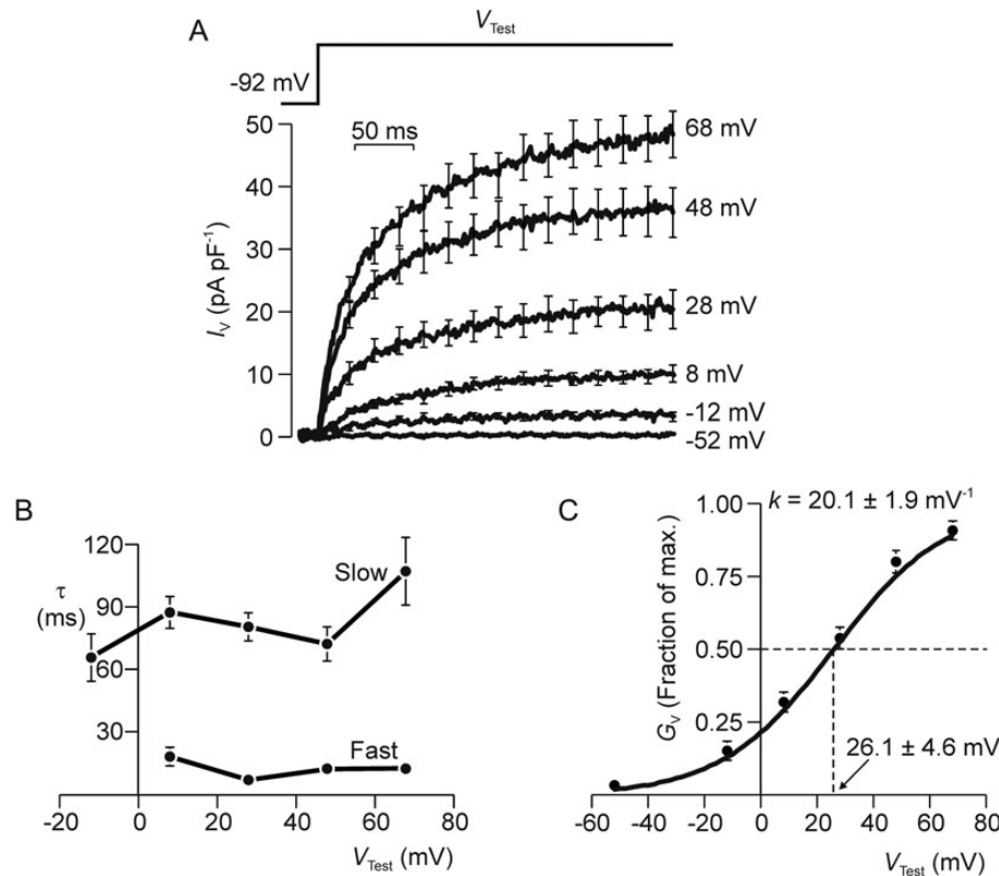
Figure 5 Kinetics of current activation. (A) Membrane currents ( n = 7-16 ) evoked by maintained voltage steps to a series of test potentials ( V_{\text{Test}} ). (B) The responses to step depolarization consistently followed time courses that were very accurately modelled as the sum of two exponential processes. The time constants ( \tau ) for the fast and slow components of this response were calculated by non-linear regression and plotted against V_{\text{Test}} . All data are mean \pm s.e.m. and leak/capacitive currents were subtracted on line in order to isolate the voltage-induced component of the total membrane current ( I_v ). (C) Steady-state values of I_v were quantified over the final 50 ms of each voltage step, and used to quantify the voltage-induced increase in membrane conductance ( G_v ); the results of this analysis are plotted against V_{\text{Test}} and the solid line shows a solution to the Boltzmann Equation fitted to these data by non-linear regression. The Boltzmann constant ( k_B ) and the voltage required for half-maximal activation ( V_{50} ) are presented.
