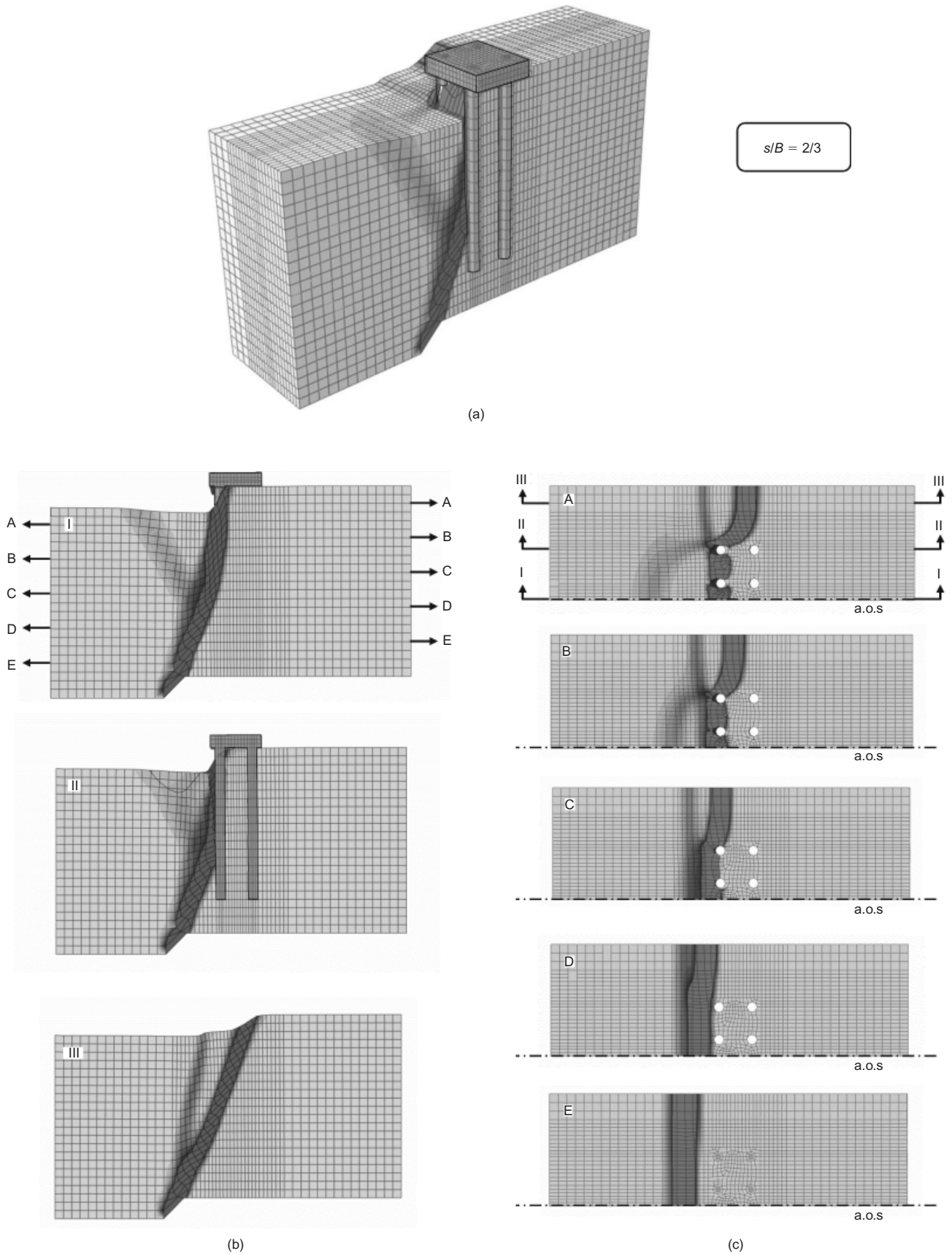
Fig. 4. Interaction of pile group with normal fault in dense sand: elastic piles, fault offset at bedrock h = 1 m, emergence of rupture in the free field at s/B = 2/3 : (a) 3D deformed finite-element mesh with superimposed plastic strain contours; (b) three vertical sections: I through the centre of the group (along the x axis), II through the edge row of piles, III in the free field, 4.5d away from the group; (c) five horizontal sections, ranging from A just below the ground surface down to E just below the pile tips (a.o.s.: axis of symmetry)
