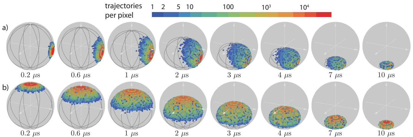
Figure 4: Statistics of quantum trajectories. Distributions of the qubit states along 10 \mu\text{s} -long trajectories for a qubit initially in |+x\rangle (a) and |e\rangle (b). The number of trajectories reaching each cubic cell of side 0.04 is encoded in color, out of a total of 3 millions. White arrows go from -1 to +1 along \sigma_{x,y,z} and the Bloch sphere is colored in gray. Meridians of the spheroid spanned by Eq. (5) are also shown.
