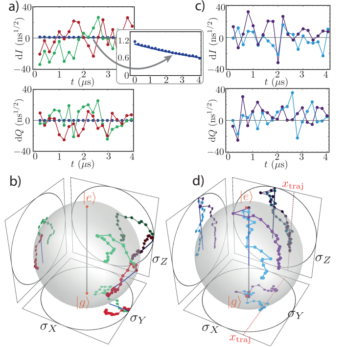
Figure 2: Quantum trajectories. a) Each panel displays two different measurement records of one quadrature of the fluorescence field for a qubit initially in |+x\rangle . Actual measurements are shown as red and green dots linked by straight lines for clarity. The blue dots correspond to the average record on all experiments, and the blue line corresponds to an exponential fit of these dots in e^{-\gamma_1 t/2 - \gamma_\phi t} . A zoom in is shown as an inset. Measurements of dI and dQ are normalized by an overall prefactor so that their variance is dt [28]. b) Quantum trajectories followed by the qubit under relaxation represented in the Bloch sphere for the measurement records shown in Fig. 2a. The Bloch vector (x, y, z) corresponds to the state \rho = (\mathbf{1} + x\sigma_x + y\sigma_y + z\sigma_z)/2 and the black circles set the scale of the Bloch sphere extrema. The trajectories are obtained by solving numerically Eq. (2) and are shown as dots linked by straight lines both in the sphere and in the three projections along x , y and z . Colors identify which record of Fig. 2a is used. A blue line shows the average evolution without monitoring ( \eta = 0 ). c,d) Same representations for two realizations starting from |e\rangle . They were arbitrarily selected to end up in a state with similar Bloch coordinate x_{\text{traj}} = 0.42 \pm 0.02 as indicated by a dashed red line.
