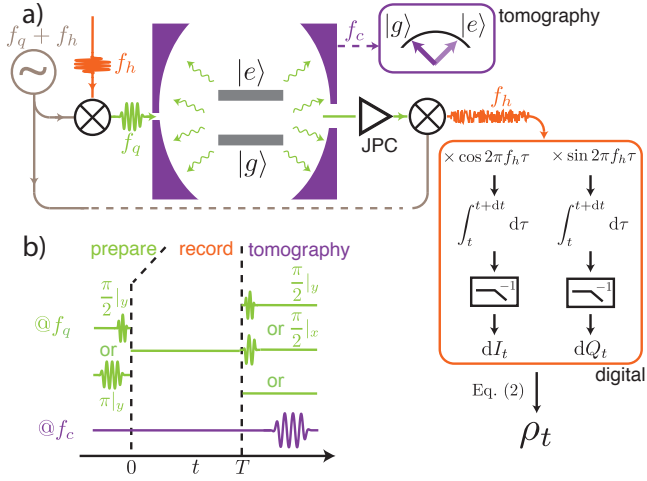
Figure 1: Scheme of the experiment. a) The fluorescence field of a superconducting qubit in an off-resonant cavity is recorded using a heterodyne detection setup from time 0 to T . Following amplification by a Josephson Parametric Converter (JPC), the signal is downconverted to f_h = 100 MHz and numerically demodulated and integrated on time steps dt = 200 ns into its two quadratures dI and dQ . The rectangular symbols represent the correction of finite detection bandwidth in the setup [28]. The quantum trajectory \{\rho_t\} is then computed using Eq. (2). A single local oscillator at f_q + f_h is used for qubit manipulation and downconversion of the fluorescence signal. The transmission at cavity frequency f_c = 7.8 GHz is used to independently readout the qubit at time T [28]. b) Pulse sequence. At time 0, the qubit is prepared in |+x\rangle (resp. |+e\rangle ) with a 52 ns (resp. 104 ns) rotation pulse around \sigma_y . The fluorescence record is acquired for a duration T ranging from 0 to 10 \mu s. The state is then projectively readout along one of the three Pauli operators using a pulse at frequency f_c preceded by a rotation pulse around \sigma_y , \sigma_x , or no pulse.
