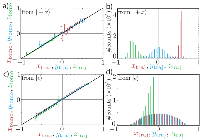
Figure 3: Tomography versus quantum trajectories.
