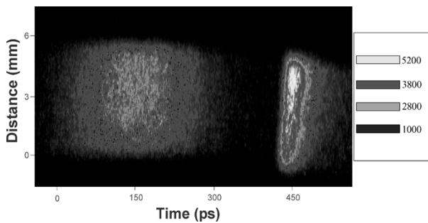
Fig. 6. Streaked slit camera image showing the plasma emission filtered by a 3.4- \mu\text{m} aluminum filter from the background and main laser pulses incident onto a nickel target. Relative intensity scale is also shown.
