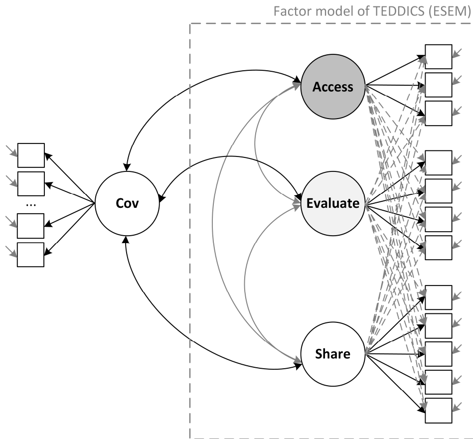
Figure 2. Exploratory structural equation model describing the relations between TEDDICS and another construct (Covariate, Cov ). Access = Accessing digital information, Evaluate = Evaluating digital information, Share = Sharing and communicating digital information.
