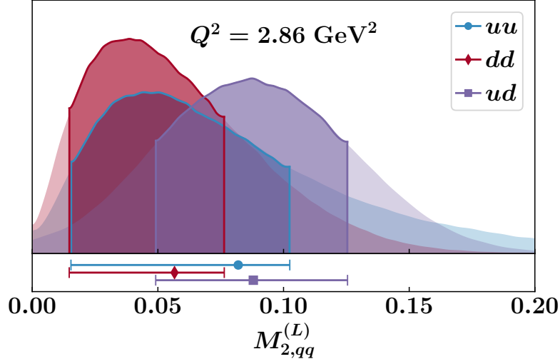
Figure 11. Density plots of the posterior distributions for the lowest M_2^{(L)} moments for uu , dd , and ud contributions. We show the results for Q^2 = 2.86 \text{ GeV}^2 from the 48^3 \times 96 ensemble. 68% credible regions of the highest posterior density are indicated by the darker regions on the density plot and shown on the lower panel along with the means of the distributions.
