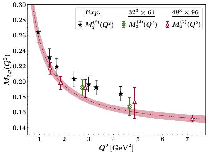
Figure 2. Q^2 dependence of the lowest moments of F_2 for the proton. Filled stars are the experimental Cornwall-Norton moments of F_2 taken from Table I of Ref. [38]. We have assigned a 5% error to the experimental moments as indicated in Ref [38]. Red band is the fit (Eq. (20)) to the 48^3 \times 96 data points.
