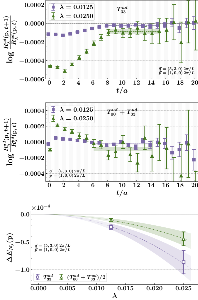
Figure 7. Same as Fig. 4 but for the purely higher-twist ud piece. We show the results obtained on the 48^3 \times 96 ensemble for the (\mathbf{p}, \mathbf{q}) = ((1, 0, 0), (5, 3, 0)) 2\pi/L pair. Energy shifts for the T_{00} + T_{33} combination have been rescaled by a factor of 0.5 on the bottom plot for clarity.
