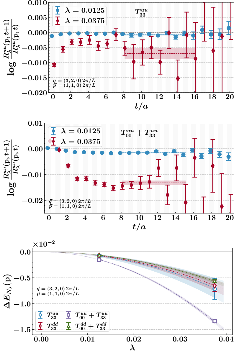
Figure 4. Top to bottom: Effective mass plots for the correlator ratios of the amplitudes T_{33} and T_{00} + T_{33} , and the corresponding fits in \lambda -space, respectively. Shaded regions on the correlator ratio plots depict the fit windows and extracted energy shifts with their 1\sigma uncertainty bands. Shaded curves on the \lambda -fit plots indicate the fit curves and their 1\sigma uncertainties. We show the results for \omega = 0.77 ( \mathbf{p} = (1, 1, 0) 2\pi/L ) for \mathbf{q} = (3, 2, 0) 2\pi/L obtained on the 48^3 \times 96 ensemble.
