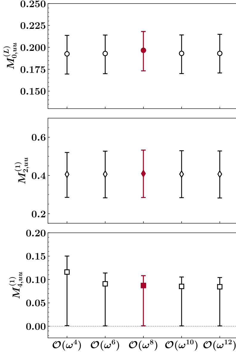
Figure 10. Stability plots for the lowest moments obtained on the 48^3 \times 96 ensemble at Q^2 = 4.86 \text{ GeV}^2 for the uu contribution only. dd and ud contributions behave similarly. We show M_0^{(L)} (top) that is directly proportional to the lowest moment of F_2 , and the lowest two moments, M_2^{(1)} (middle) and M_4^{(1)} (bottom) of F_1 with respect to the number of terms kept in the fit polynomials. Colour filled symbols indicate the values that we pick.
