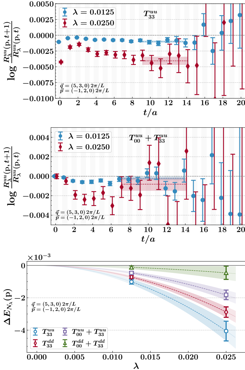
Figure 6. Same as Fig. 4 but for \omega = 0.06 ( \mathbf{p} = (-1, 2, 0) 2\pi/L ) for \mathbf{q} = (5, 3, 0) 2\pi/L .
