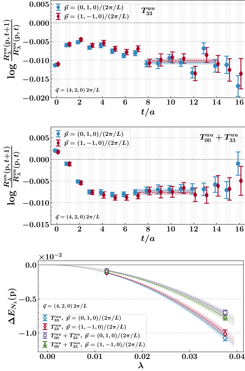
Figure 9. Top to bottom: Correlator ratios of the amplitudes T_{33} and T_{00} + T_{33} for \lambda = 0.0375 , and the corresponding fits in \lambda -space, respectively, for two different \mathbf{p} momenta that give \omega = 0.2 at fixed \mathbf{q} = (4, 2, 0) 2\pi/L . See the caption of Fig. 4 for the explanation of shaded regions. We show the results for the uu piece obtained on the 48^3 \times 96 ensemble.
