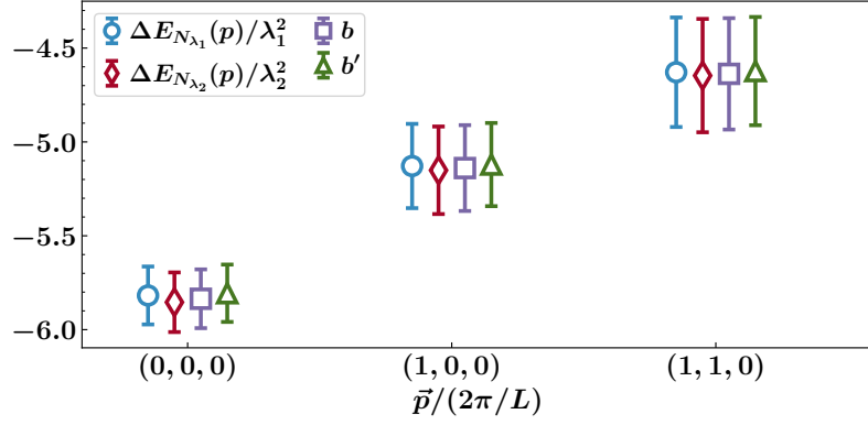
Figure 8. The coefficient of the quadratic term in Eq. (18) determined in four different ways (see text). b and b' are the quadratic coefficients obtained from a purely quadratic, f(\lambda) = b\lambda^2 , and a quadratic-plus-quartic, g(\lambda) = b'\lambda^2 + c\lambda^4 , fit. We show the results for the uu piece obtained on the 48^3 \times 96 ensemble at fixed \mathbf{q} = (5, 3, 0) 2\pi/L .
