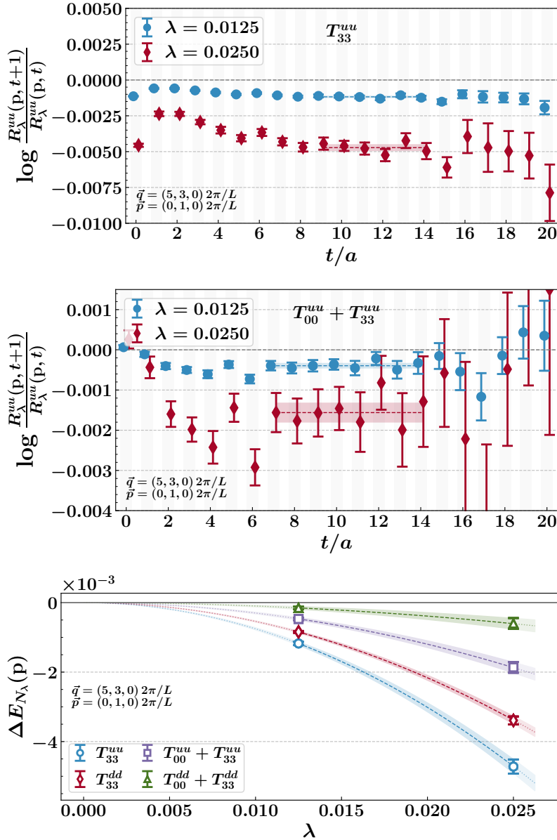
Figure 5. Same as Fig. 4 but for \omega = 0.18 ( \mathbf{p} = (0, 1, 0) 2\pi/L ) for \mathbf{q} = (5, 3, 0) 2\pi/L .
