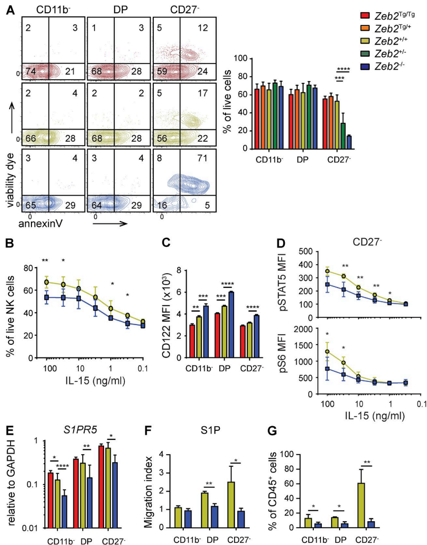
Figure 2. Zeb2 is indispensable for survival of mature NK cells and for their exit from the BM.
