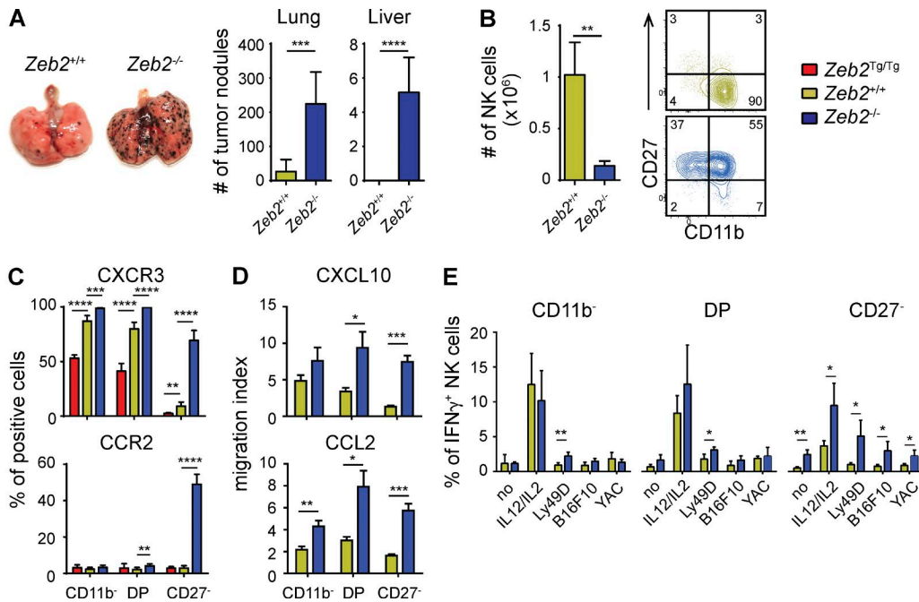
Figure 3. NK-Zeb2 -/- mice are highly susceptible to B16F10 melanomas. (A) NK-Zeb2 -/- and littermate control (NK-Zeb2 +/+ ) mice were i.v. injected with 200,000 B16F10 melanoma cells. Mice were sacrificed 12 d later, and tumor nodules in lung and liver were counted. n = 6 representative for two independent experiments. (B) Absolute lung NK cell numbers of unchallenged NK-Zeb2 -/- and littermate control (+/+) mice. FACS plots show a representative CD11b/CD27 profile of gated CD3 + CD122 + NK1.1 + NK cells as determined by flow cytometry. n \geq 3 representative for two independent experiments. (C) Flow cytometry measurement of the expression of CXCR3 and CCR2 by gated splenic NK cell (CD3 + CD122 + NKp46 + ) subsets. Results show the percentage \pm SD of positive cells among NK cells of the indicated subset. n > 5 representative of at least two independent experiments. (D) Chemotaxis assay of spleen NK cells of the indicated genotype using CXCL10 and CCL2. n = 4-8 pooled from two independent experiments. (E) Lung lymphocytes were isolated from day 1 B16-bearing animals and restimulated ex vivo for 4 h in the indicated conditions in the presence of GolgiStop. Their production of IFN- \gamma was measured using flow cytometry. n = 4 in each group, representative for two independent experiments. All bar graphs represent the mean \pm SD results. *, P < 0.05 ; **, P < 0.01 ; ***, P < 0.001 ; ****, P < 0.0001 (Student's t test).
