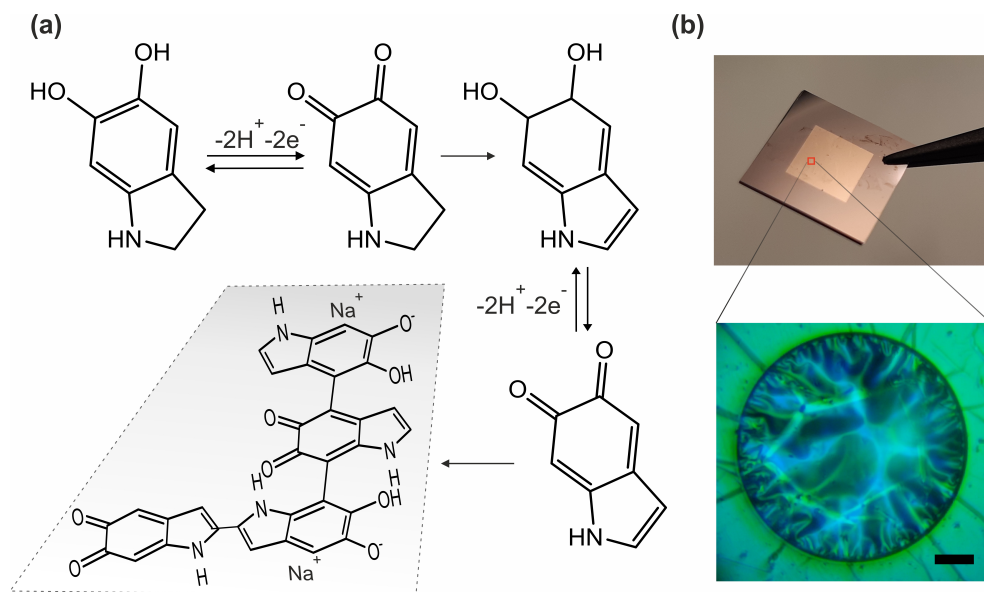
Figure 1: (a) The synthesis procedure of PDA with hydroxyl indole-like structures. 34 (b) Optical images of the \text{Si}_3\text{N}_4 membrane grid covered with the PDA film (upper panel) and a free-standing PDA membrane (lower panel). The scale bare is 10 \mu\text{m} .
