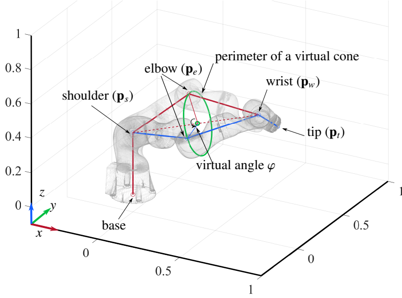
Figure 3: Two configurations of the KUKA iiwa at the same pose are illustrated in red and blue lines. The green rim indicates the virtual movement of the elbow position w.r.t the specific end-effector pose. The red lines and blue lines illustrate the robot at the arm angle \varphi = 0 and \varphi = 95^\circ , respectively.
