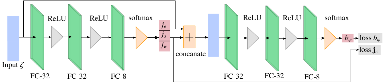
Figure 7: Architecture of the proposed NN for learning the joint configuration \mathbf{j}_c and the bin index b_\varphi of the virtual angle \varphi .
