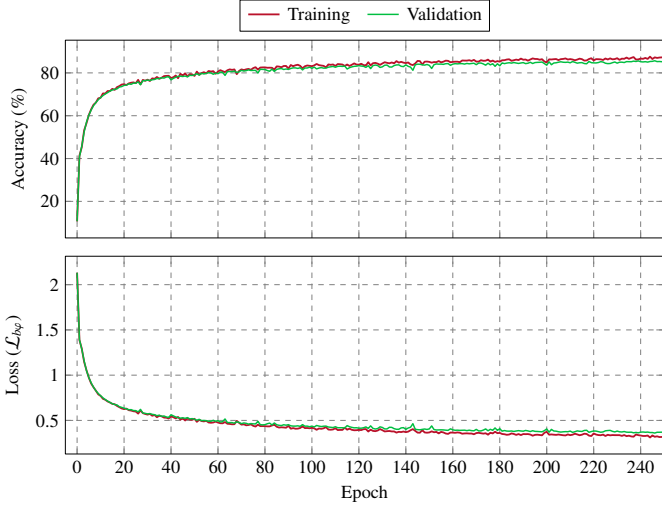
Figure 9: Training and validation accuracy of the bin index b_\varphi .
