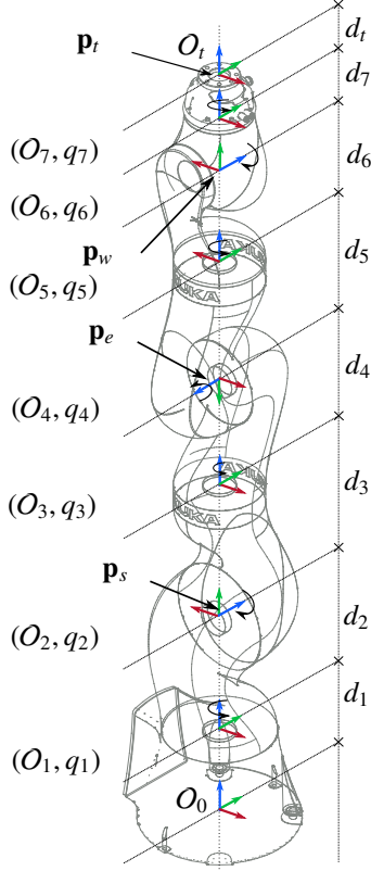
Figure 2: Schematic drawing of the robot KUKA LBR iiwa. The x -, y -, and z -axis of each coordinate frame are shown as red, green, and blue arrows, respectively.
