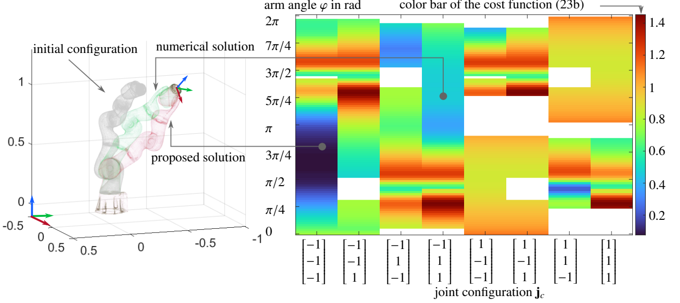
Figure 5: The color map of the cost function (23b) for the initial configuration of the robot \mathbf{q}_0 (in gray color) and the position of the end effector (the RGB triad) is shown on the right-hand side of this figure. The white color regions depict infeasible joint configurations. The robot target configuration \mathbf{q}_{t_F} computed by the proposed NN is shown in red color on the left-hand side. This achieves a very small value of the cost function (23b) ( \approx 0.0717 ). The target robot configuration calculated using the numerical method [5] is depicted in green. The cost of this configuration is approximately 0.54.
