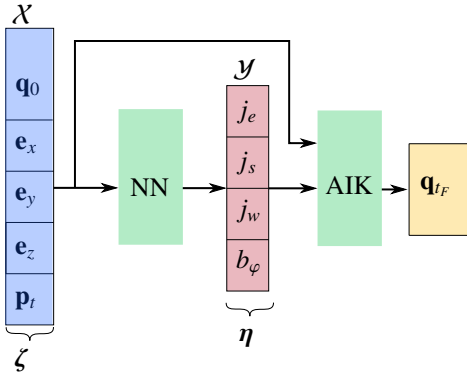
Figure 6: Overview of the proposed framework for learning the redundancy parameters.
