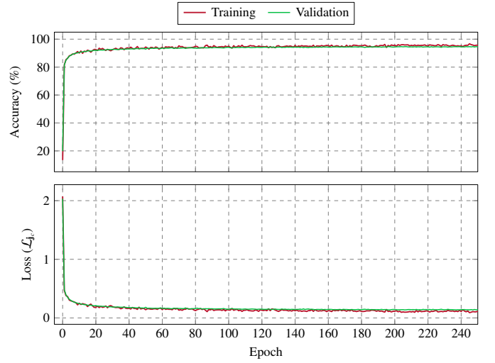
Figure 8: Training and validation accuracy of the joint configuration \mathbf{j}_c .
