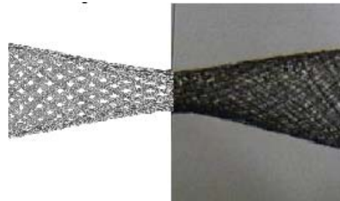
Figure 6: The numerical model (left) is able to predict the shape of the stent when loaded experimentally (right) to determine the central radial stiffness.
