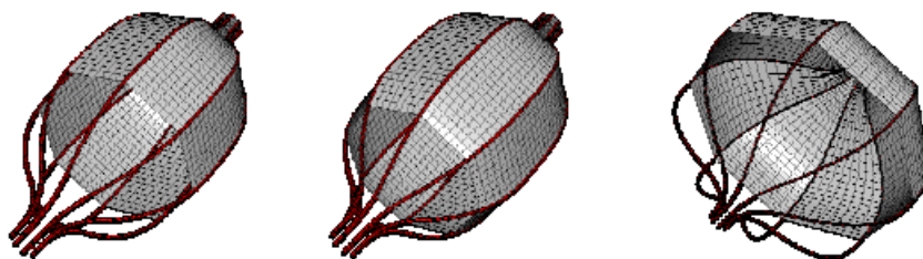
Figure 7: Design variants of the Angioguard model: original 4 mm device with 50% membrane coverage (left), 70% membrane covered 4 mm filter (middle), 8 mm device with 50% membrane coverage (right).
