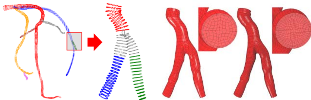
Figure 8: Geometrical data from coronary angiography (left), coarse and fine mesh models (right).
