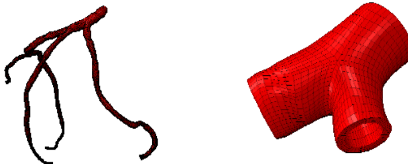
Figure 9: Reconstruction of the wall sections from the lumen and parametric hexahedral mesh generation.
