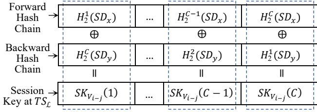
Fig. 5: Hash chains used to generate SK_{V_{i-j}}(TS_L) .
