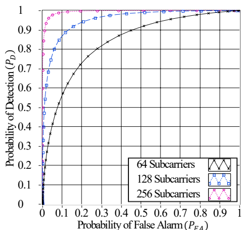
Fig. 9: P_D versus P_{FA} at R = 70\% , M = 1 , \text{SNR} = 5 dB, and number of subcarriers N = \{64, 128, 256\} subcarriers.
