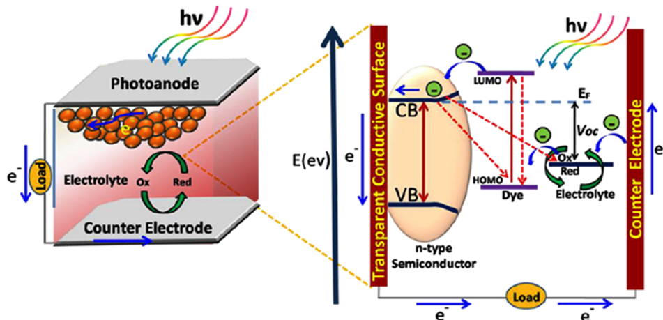
FIG. 2. Schematic representation of the working principle of a DSSC device.
