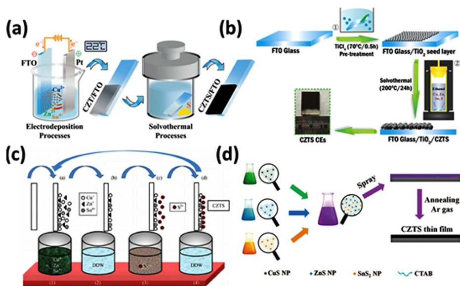
FIG. 11. (a) Schematic illustration of the fabrication processes of the CZTS counter electrode via electrodeposition and further solvothermal process. “Reproduced with permission from Chen et al. , Green Chem. 8 , 2793 (2016). Copyright 2016 The Royal Society of Chemistry.” (b) Schematic illustration of the fabrication processes of the CZTS counter electrode. “Reproduced with permission from Chen et al. , ACS Sustainable Chem. Eng. 3 , 2652 (2015). Copyright 2015 American Chemical Society.” (c) Schematic diagram of SILAR technique for the deposition of CZTS: beaker 1 contains cationic precursors, beaker 3 contains anionic precursor and beakers 2 and 4 contain double distilled water (DDW). “Reproduced with permission from Shinde et al. , Mater. Res. Bull. 47 , 302 (2012). Copyright 2012 Elsevier.” (d) Schematic diagram of the preparation of CZTS solution using metal sulfides with cetyltrimethyl ammonium bromide (CTAB) as the capping ligand. “Reproduced with permission from Li et al. , RSC Adv. 4 , 26888 (2014). Copyright 2014 The Royal Society of Chemistry”.
