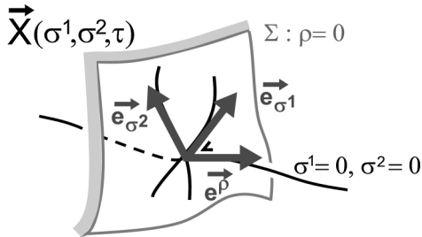
FIG. 1. Gaussian normal coordinates near the wave front.
