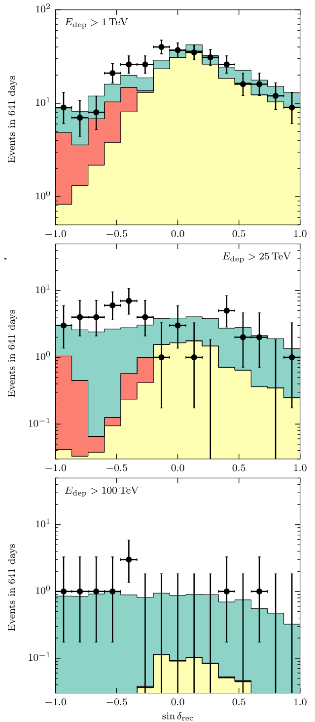
FIG. 9 (color online). Zenith angle distribution of events depositing more than 1, 25, and 100 TeV (points) with the best-fit combination of atmospheric and astrophysical contributions from Table I, using the same color scheme as in Fig. 8. At the lowest energies the sample is concentrated at the horizon, as expected from conventional atmospheric neutrinos. The astrophysical component contributes significantly to the sample above 25 TeV, and the bulk of the sample is down-going. By 100 TeV only the astrophysical component remains, and the up-going flux is suppressed by absorption in the Earth.
