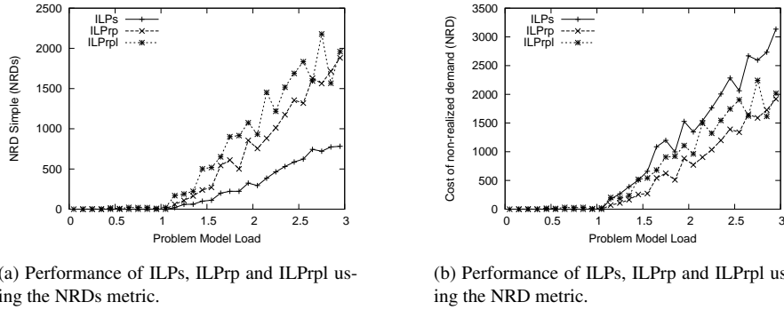
Fig. 8: Performance of ILPs, ILPrp and ILPrpl using different quality evaluation metrics using the VC scenario.
