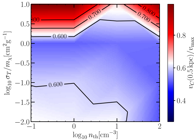
Figure 5. Same as upper panel of Fig. 4, but after 4 Gyr of simulation time.
