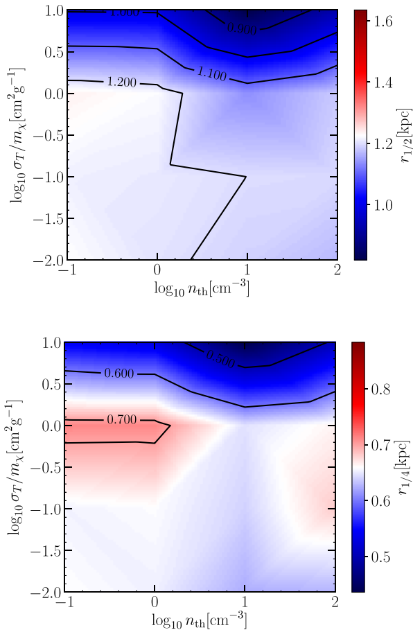
Figure 6. The galaxy half (stellar) mass radius r_{1/2} (top panel) and quarter (stellar) mass radius r_{1/4} (bottom panel) as a function of \sigma_T/m_\chi and n_{th} , measured after 3 Gyr. As in Fig. 4, the parameter space shown is filled by interpolation across the 16 simulations in our suite. Contour lines indicate degeneracies (i.e. equal values of either r_{1/2} or r_{1/4} ) in parameter space. Notice that the half-mass radius in all cases is larger than the typical core radius of \sim 0.7 kpc found in Fig. 3. Thus, the impact of different core formation mechanisms is much more apparent in the quarter mass radius.
