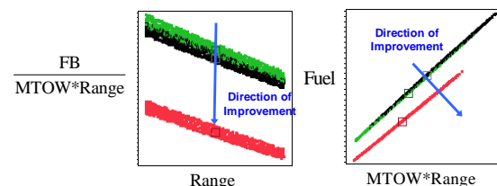
Fig. 13 Examples of Metric-CPs with MTOW Term
