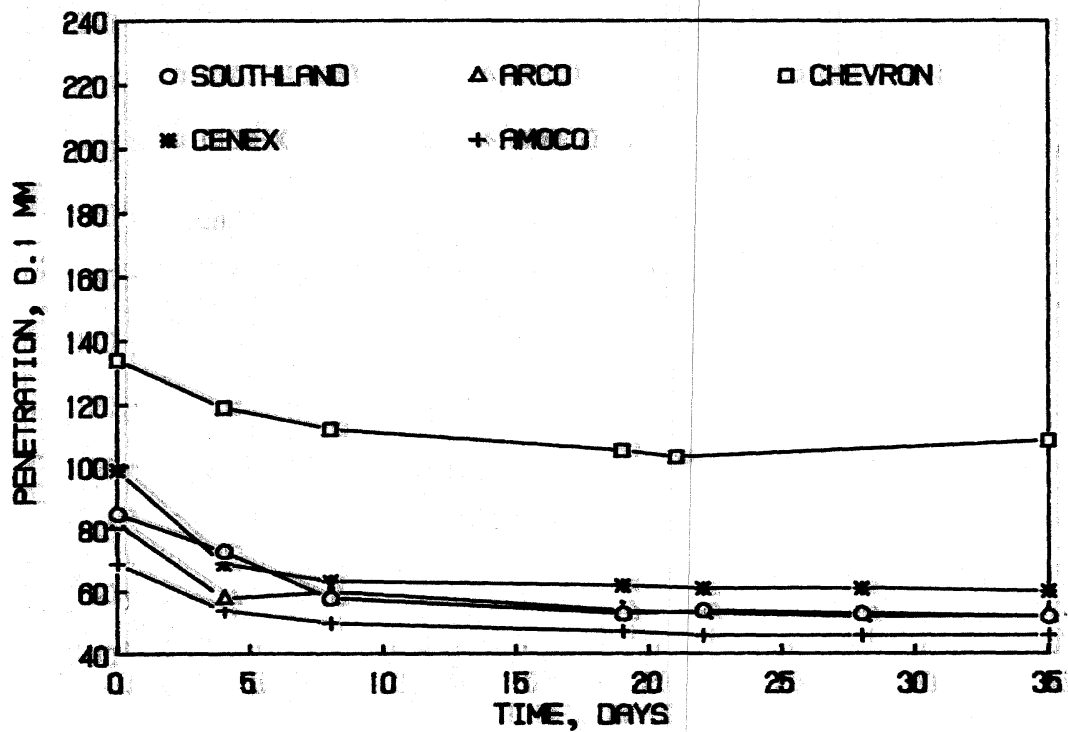
Figure 16. Second data set - SEA penetration versus time.
