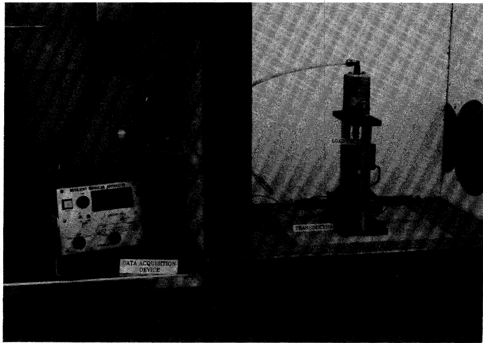
Figure 1. Retsina Mark V diametral resilient modulus apparatus.
