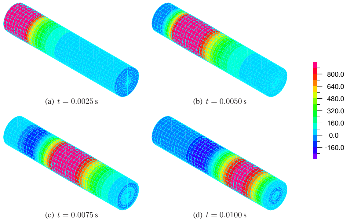
Figure 2: Wave propagation in the straight elastic tube. Pressure contours on the fluid-structure interface.
