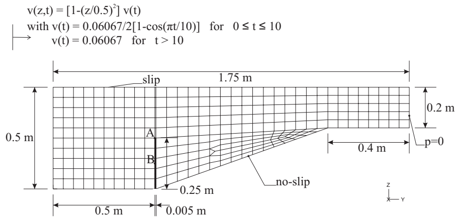
Figure 8: Flexible restrictor in the converging channel. Geometry, boundary conditions and mesh for the solid (black) and fluid (white) model.
