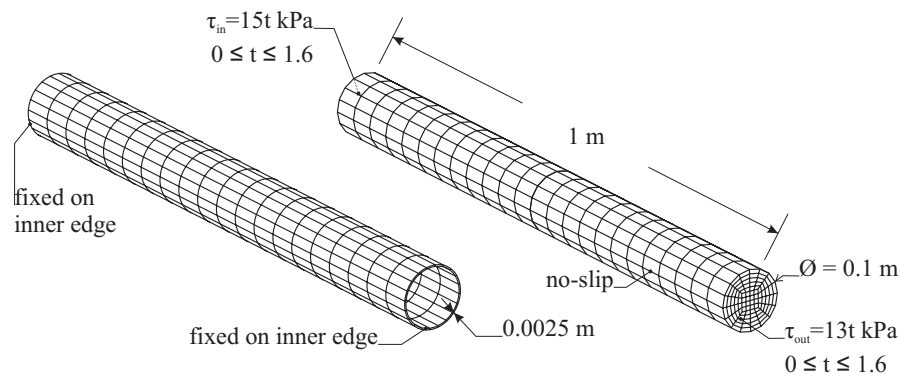
Figure 3: Mass conservation test. Geometry, boundary conditions and mesh for the solid (left) and fluid (right) model.
