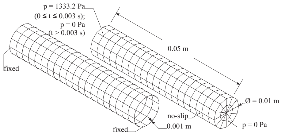
Figure 1: Wave propagation in the straight elastic tube. Geometry, boundary conditions and coarsest mesh for the solid (left) and fluid (right) model.
