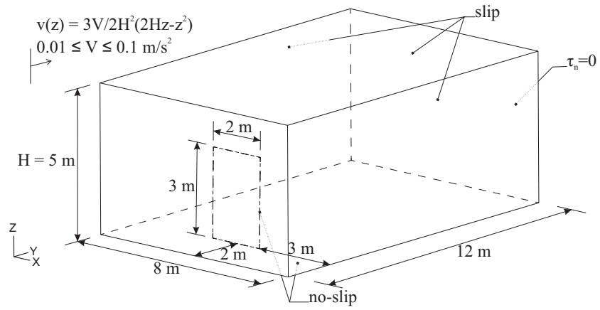
Figure 7: Shell in steady-state cross-flow test. Geometry and boundary conditions for the solid and fluid model.
