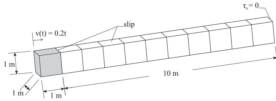
Figure 5: Strong coupling test. Geometry, boundary conditions and coarsest mesh for the solid (grey) and fluid (white) model. The solid is confined to stay in the channel.
