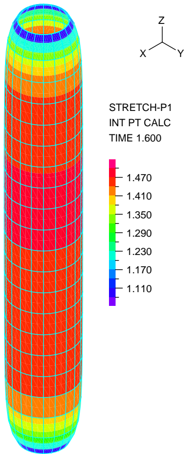
Figure 4: Mass conservation test. Maximum principal stretch
