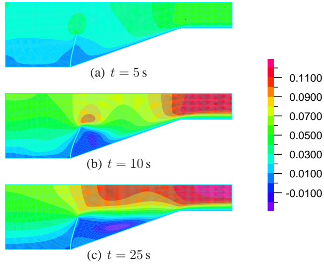
Figure 9: Flexible restrictor in the converging channel. Horizontal velocity.
