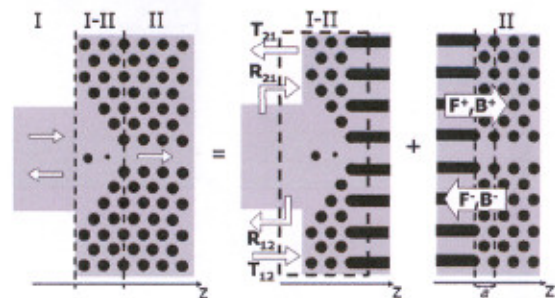
FIG. 1. Schematic of the proposed semianalytic approach for analyzing a structure formed by a dielectric waveguide coupled to a semi-infinite photonic crystal (PhC) waveguide by using an especially designed two-defects configuration placed within a PhC taper. T_{12} , R_{21} , T_{21} , and R_{12} are the transmission and reflection matrixes calculated in mediums I–II while F_+ ( F_- ) and B_+ ( B_- ) are the forward and backward components of the forward (backward) propagating Bloch modes calculated at the interface layer between mediums I–II and medium II, which corresponds to a fixed cut position within the lattice period, a , of the PhC. The z axis indicates the propagation direction.
