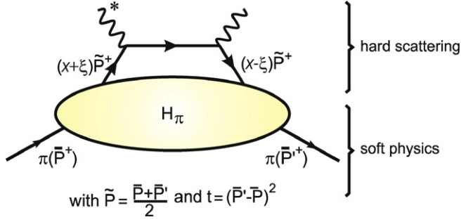
Fig. 2. Feynman diagram of DVCS, with definition of the kinematical variables x , \xi and t .
