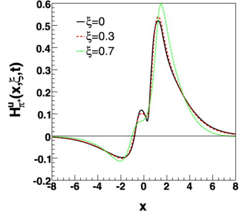
Fig. 4. The pion GPD H_{\pi^+}^u as a function of x , calculated in the Bonn constituent quark model at t = -0.1 \text{ GeV}^2 . Results are shown for \xi = 0 (solid line), \xi = 0.3 (dashed line) and \xi = 0.7 (dotted line).
