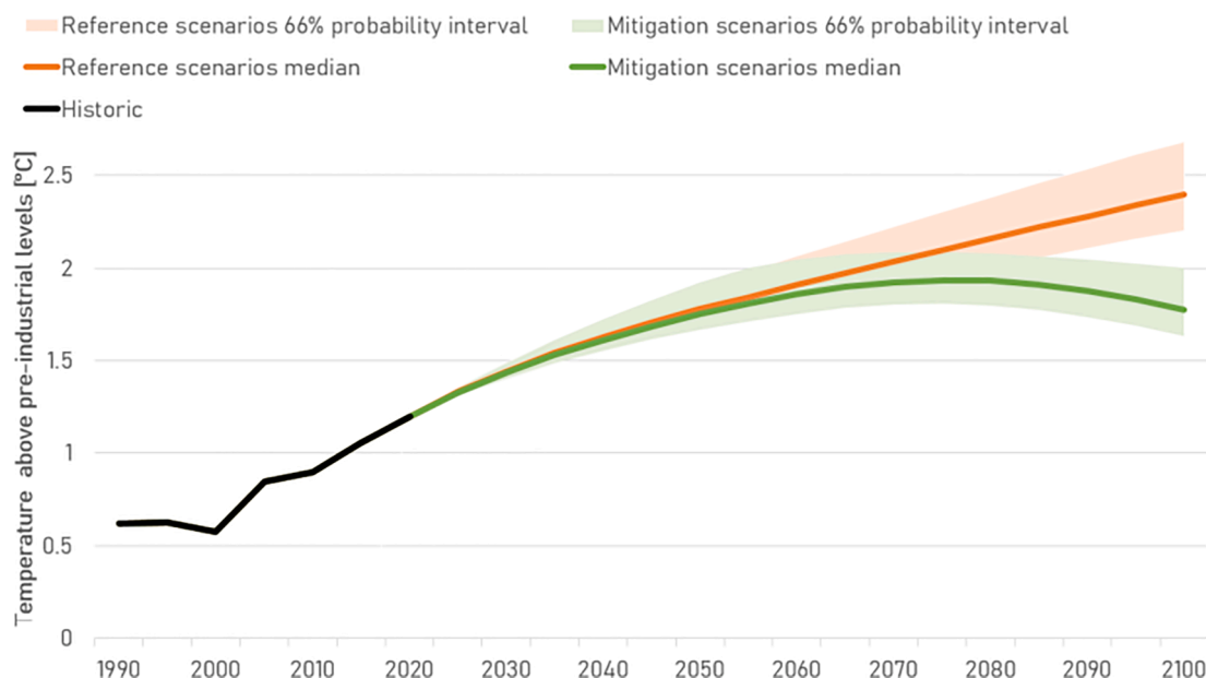
Fig. 3. Global mean temperature evolution for mitigation and reference scenarios with 66% probability range. Non-modelled data (“Historic”) taken from GISTEMP Team (2021) and Lenssen et al. (2019).
